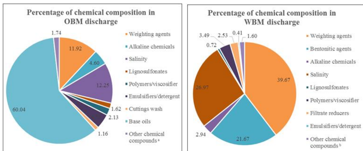
Fig. 1 Percentage of individual chemical constituents present in OBM and WBM discharge adapted from Hudgins [31].
