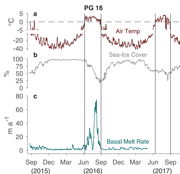
Fig. 3. (a) AWS air temperature time series from PG 16 smoothed with a 2-day running median filter. (b) Daily SSM/I sea ice cover near PGIS ( 81^{\circ}\text{N} – 82^{\circ}\text{N} , 60^{\circ}\text{W} – 67^{\circ}\text{W} ) from NSIDC archives at 25 km resolution (Steffen and Schweiger, 1991). (c) Basal melt rate time series from PG 16 smoothed with a 2-day running median filter. Grey-shaded air temperatures come from updated output of the 1 km resolution downscaled RACMO2.3 model (Noël and others, 2016) for PGIS. Black vertical lines indicate the 2016 and 2017 summer seasons when air temperatures exceeded 0^{\circ}\text{C} (grey dashed line).
