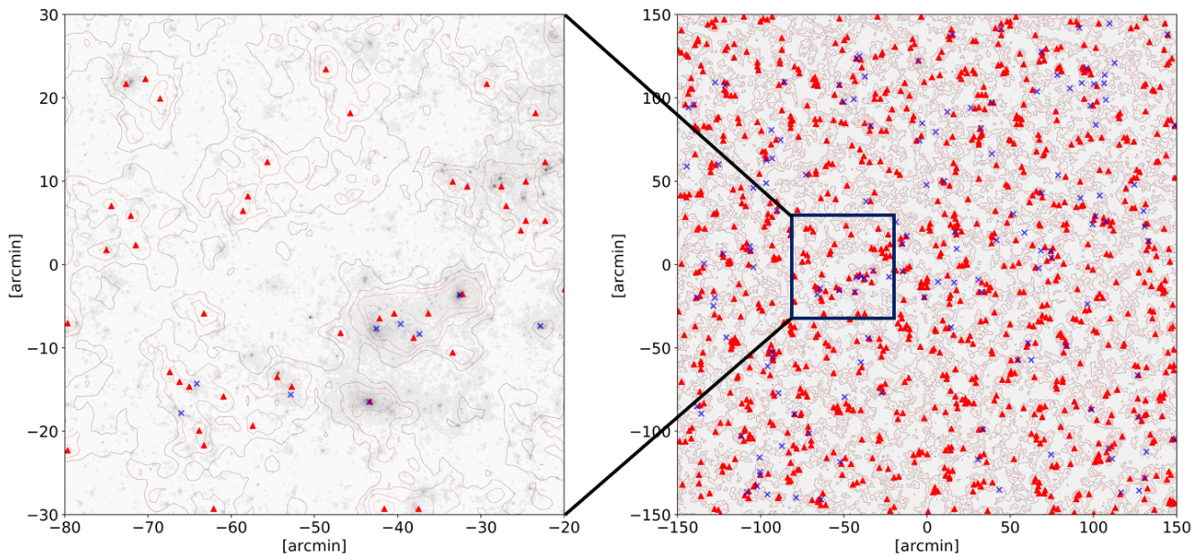
Figure 2. A 60 \times 60 \text{ arcmin}^2 sub-region of a 5 \times 5 \text{ deg}^2 aperture mass map for source number density 9 \text{ gal/arcmin}^2 . The aperture size is 12.5 \text{ arcmin} , and the S/N contour lines are plotted from 0 with an increment of 1. The field in grey scale in the background is the light-cone convergence map, and the cross marks are the locations of clusters from the BAHAMAS friends-of-friends catalogues, where the lowest mass cut is 10^{14} M_{\odot} and the upper limit redshift cut for the clusters is at z=0.5 . The triangles are the peak locations above S/N=2 .
