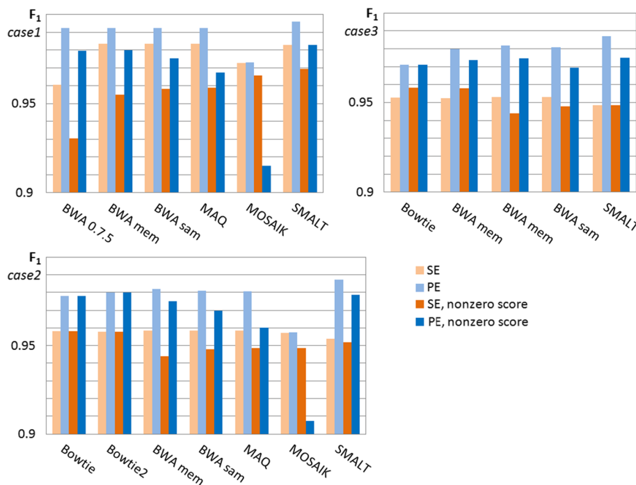
Fig. 7 F1 scores. All reads – light colour bars, non-sero reads (“reliable”) – dark colour bars
