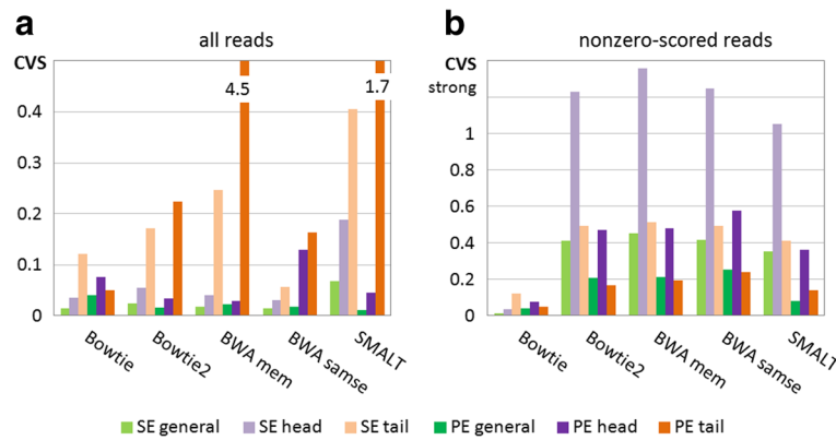
Fig. 6 Coefficients of variation of the sample, case3. Panel labels: general (total) CVS are marked in green, head CVS - in mauve, tail CVS - in brown. SE are shown with light colour bars, PE - with dark colour bars
