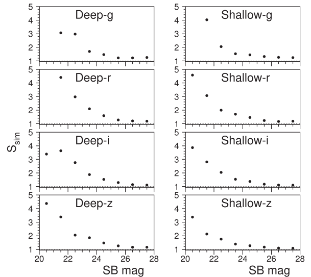
Figure 2. Simulated uncertainty scale, \hat{S}_{\text{sim}} , as a function of local surface brightness mag (SB mag). Each panel indicates the set of fields and passband. Left-hand panels are for the deep SN fields (depth per visit \sim 24.5 ); right-hand panels are for shallow SN fields (depth per visit \sim 23.5 ).
