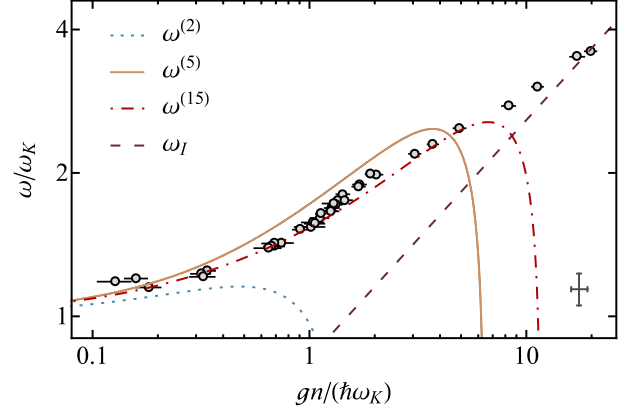
FIG. 4. Crossover from single-particle excitations to sound waves. We plot \omega/\omega_K as a function of the interaction strength, now parametrized by gn/(\hbar\omega_K) . Here we assume L = 26 \mu\text{m} and R = 16 \mu\text{m} for calculations. The x-y error bar in the bottom right corner indicates the fractional systematic uncertainties in the experimental data due to the uncertainties in the box dimensions. \omega^{(2)} is determined using Bogoliubov theory within a truncated basis of just the two lowest-energy single-particle eigenstates of zero angular momentum (see text). This scheme fails even for relatively small gn/(\hbar\omega_K) , as it does not allow for the interaction-induced changes in the shape of the condensate or the excitation mode. \omega^{(5)} , based on a truncated basis of five single-particle eigenstates, is the minimal model that allows for the shape changes. This simple model already captures most of the crossover, and using progressively larger truncated bases does not qualitatively change the result, as shown by \omega^{(15)} , which is based on 15 single-particle eigenstates. \omega_I is the sound-wave frequency, approached in the limit of large gn/(\hbar\omega_K) .
