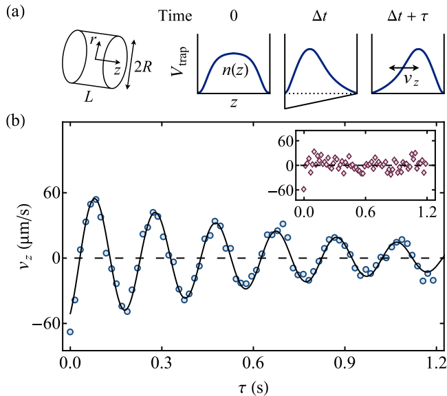
FIG. 1. Probing the lowest axial mode. (a) Illustration of the experimental protocol. We prepare a BEC of ^{87}\text{Rb} in a cylindrical box trap of length L and radius R . Initially, the trapping potential V_{\text{trap}} has a flat bottom. We then pulse a magnetic field gradient corresponding to \Delta U = k_B \times 1 nK along the box length for \Delta t = 20 ms. After a time \tau of in-trap evolution we switch off the trap and let the cloud evolve in free space for 140 ms before extracting its center of mass, which reflects the velocity on release from the trap, v_z . (b) v_z(\tau) for a BEC of N = 13(1) \times 10^3 atoms. We determine the oscillation frequency \omega using a decaying sinusoidal fit. Inset: v_z(\tau) for a noncondensed sample just above T_c , with N = 10(1) \times 10^3 .
