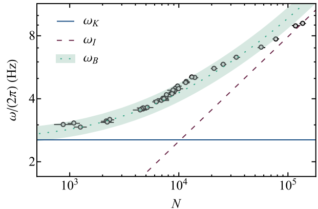
FIG. 2. Angular frequency of the lowest axial mode as a function of atom number, N . \omega_K is the mode frequency in an ideal gas, and \omega_I is the frequency of Bogoliubov sound with speed (gn/m)^{1/2} and wavelength 2L . These calculations use trap dimensions L = 26 \mu\text{m} and R = 16 \mu\text{m} . The shaded band \omega_B shows the results of numerical Bogoliubov diagonalization (see Sec. III B) accounting for the uncertainty of \pm 1 \mu\text{m} in L and R .
