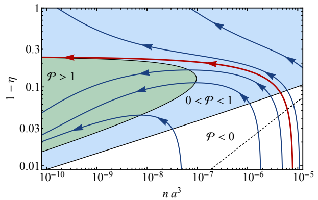
FIG. 3. Cooling and purification in a weakly interacting gas. The purification coefficient \mathcal{P} now depends on the condensed fraction \eta and the gas parameter na^3 . The evolution of the system is described by trajectories that flow either to \eta = 1 or to \eta = 0 , depending on which side of the critical trajectory \eta^*(na^3) (red line) they are. On this log-log graph the slope of the trajectories is given by \mathcal{P} - 1 [see Eq. (3)] and the background shading indicates whether instantaneously the gas purifies (green), cools without purifying (blue), or heats (white). In the regime below the dashed line, which corresponds to k_B T = 2gn , the dynamics could deviate from our results due to phononic nature of the thermal excitations.
