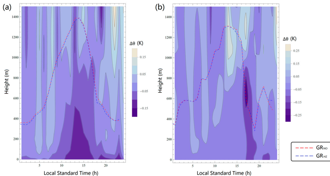
Figure 12. The same as Figure 7, but for GR NO and GR HZ (all green roofs in Hangzhou urban grids) scenarios, in (a) Hangzhou and (b) Haining (see Figure 1b).
