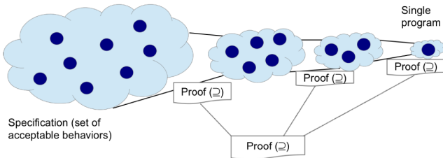
Fig. 3. Deductive program synthesis through sound refinements.
