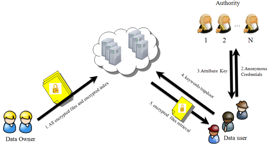
Fig. 1 Multi-authority ABKS
