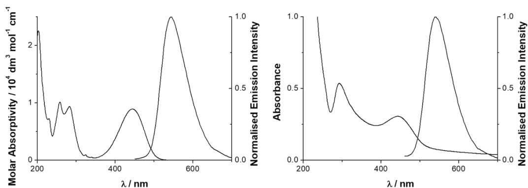
Figure 7. UV-vis. and luminescence spectra of showing Nap-1 (left) and Nap-1@ND (right) in aqueous solution.
