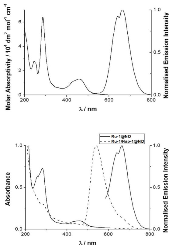
Figure 12. UV-vis. and luminescence spectra of showing Ru-1 (top), Ru-1@ND and Ru-1/Nap-1@ND (bottom) in aqueous solution.
