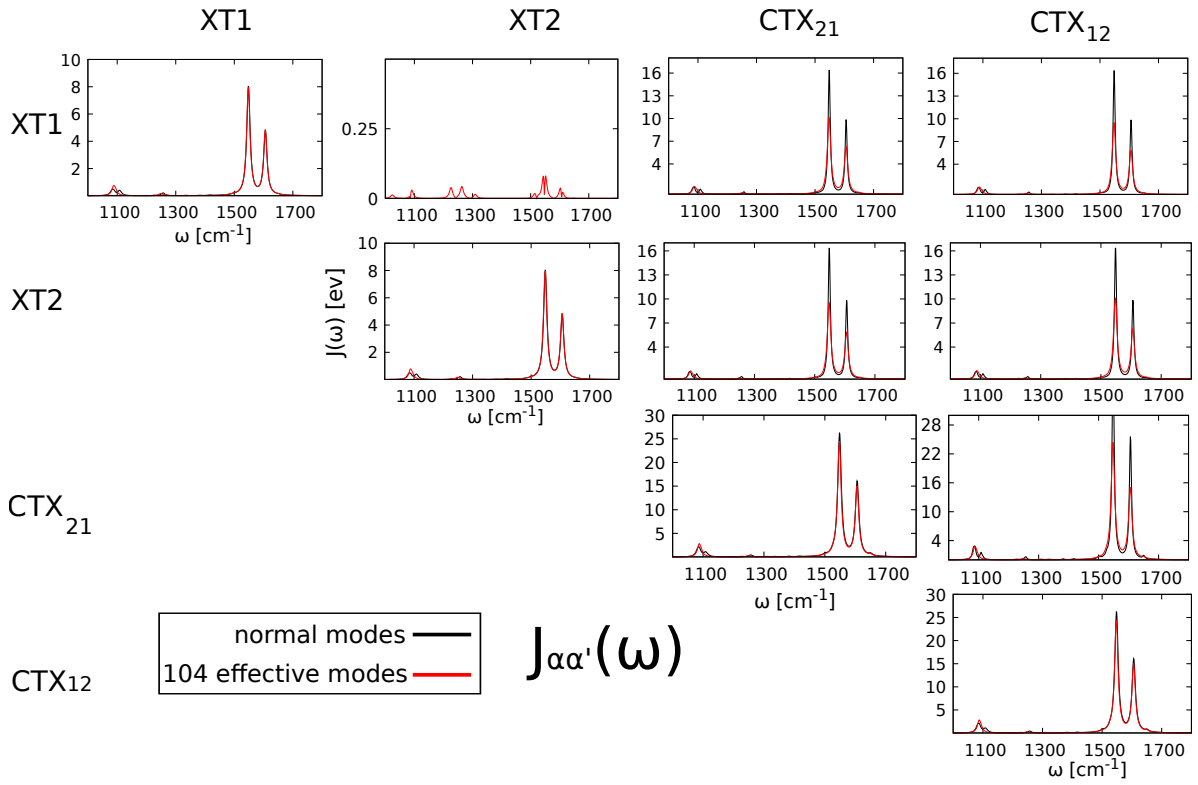
FIG. 7. For the (\text{OT4})_5 pentamer, selected elements (absolute values) of the spectral density matrix \mathbf{J}^{(k=8)} , i.e., for K = 104 effective modes, are shown (red traces), as compared with the reference spectral density in the original local NM representation (black traces). It is seen that all diagonal and off-diagonal spectral density components exhibit a similar frequency dependence, mainly characterized by the bimodal feature that is already prominent in the monomer spectral density. Note that XT-XT cross-correlations vanish by construction (and are almost zero at the k = 8 level of treatment). The convergence at the k = 8 order is very good, and of similar quality as observed in the dimer case of the preceding figure.
