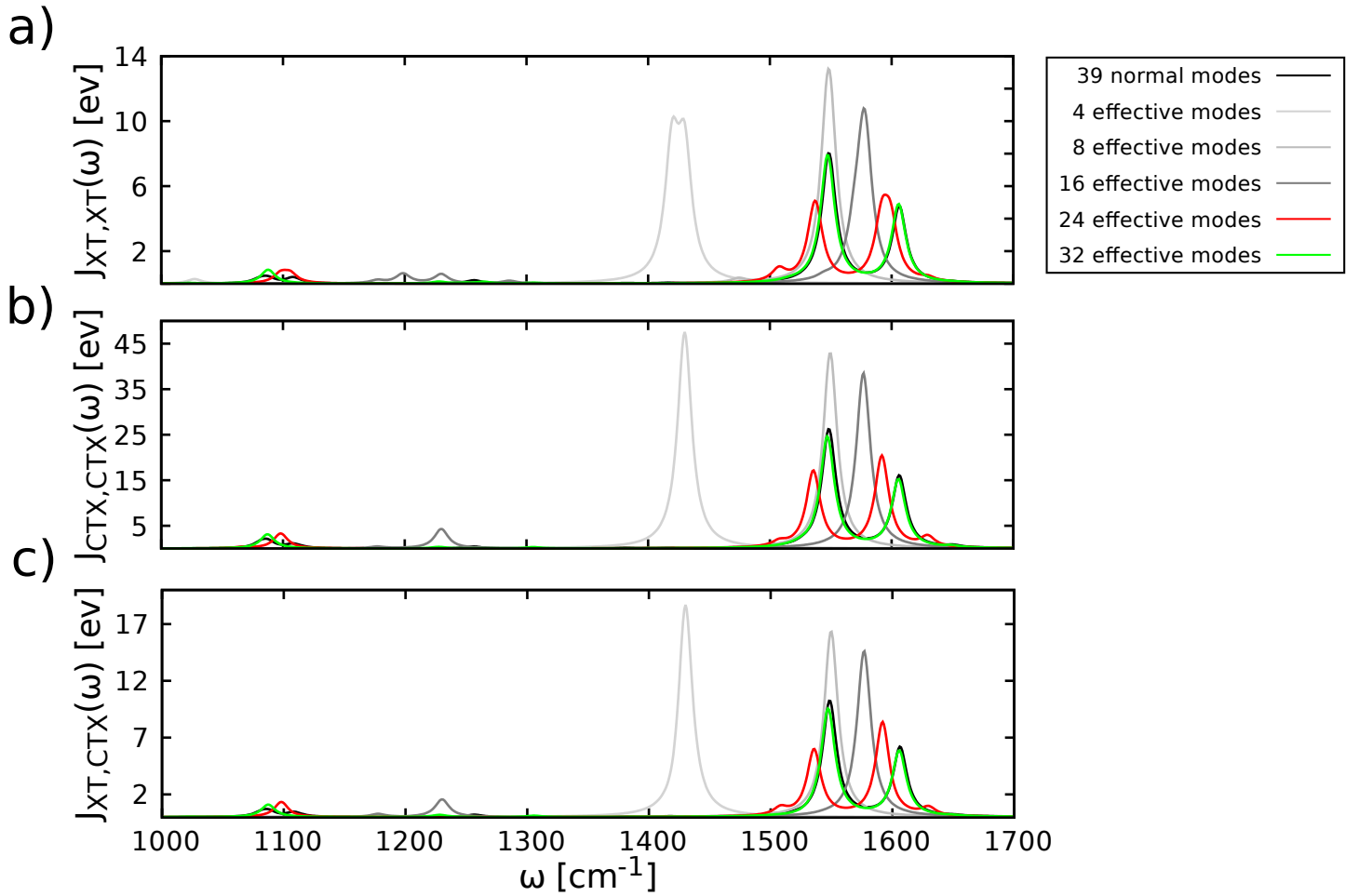
FIG. 6. For the (OT4)_2 dimer, the convergence behavior of the J_{XT,XT}^{(k)} (panel a), J_{CTX,CTX}^{(k)} (panel b), and J_{XT,CTX}^{(k)} (panel c) component spectral densities is shown for different truncation orders k of the effective-mode hierarchy, as compared with the corresponding original spectral densities in the local NM representation (shown in black). For the dimer species, N_s = 4 such that the number of effective modes is given as K = 4k . The effective mode spectral densities comprising up to 16 effective modes are drawn in grey, while those comprising 24 ( k = 6 ) and 32 ( k = 8 ) effective modes are depicted in red and green. Note the different scales for the SD components; specifically, the diagonal CTX SD takes a large values, reflecting large reorganisation effects in the CTX state. All spectral densities have been constructed with a Lorentzian broadening of \Delta = 0.1\overline{\Delta\omega} .
