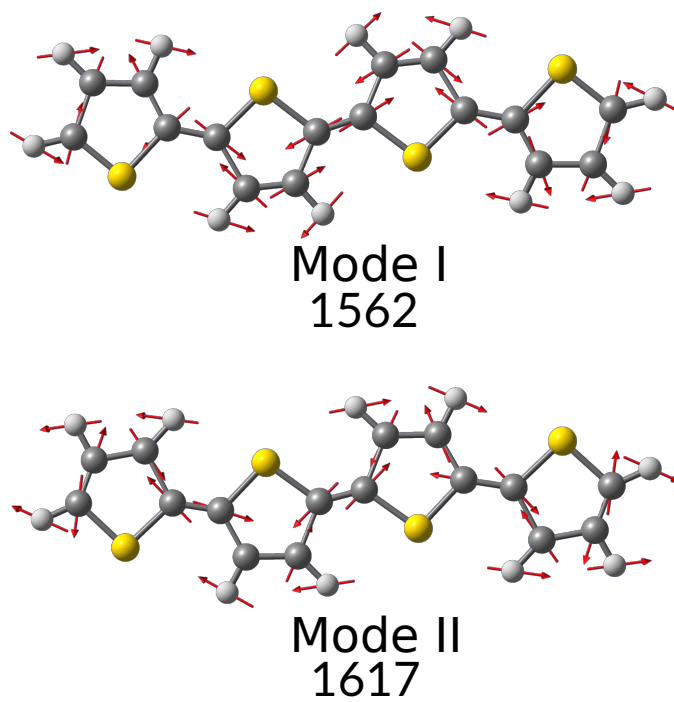
FIG. 4. Visualisation of the two most strongly coupled normal modes. Mode I corresponds to the 76th normal mode of one OT4 fragment, while Mode II corresponds to the 78th normal mode. Frequencies are indicated in \text{cm}^{-1} .
