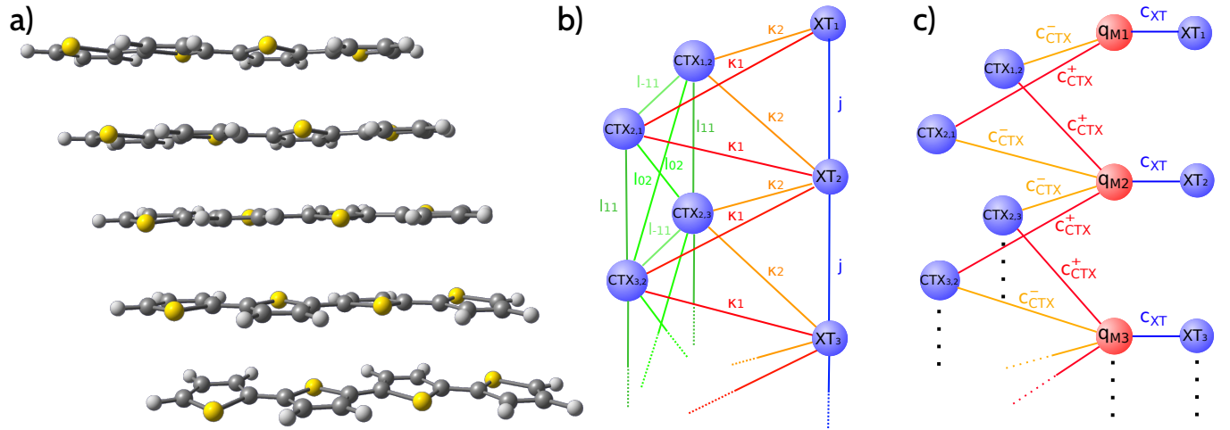
FIG. 1. a) Molecular representation of the stacked (OT4)_5 pentamer aggregate at the center of the present studies. b) Schematic representation of the electronic couplings in the aggregate system, involving XT and CTX states (blue circles). Various types of electronic couplings appearing in Eqs. (4)-(6) are marked along the edges connecting two nodes describing electronic states. c) Schematic representation of the vibronic couplings of Eqs. (14)-(15) where the monomer-specific vibrations are shown as additional nodes (red circles), the electronic states appear as in panel b (blue circles), and the relevant local ( c_{XT} ) and nonlocal ( c_{CTX}^\pm ) vibronic couplings are marked along the edges connecting two nodes of vibrational (blue) and electronic (red) type.
