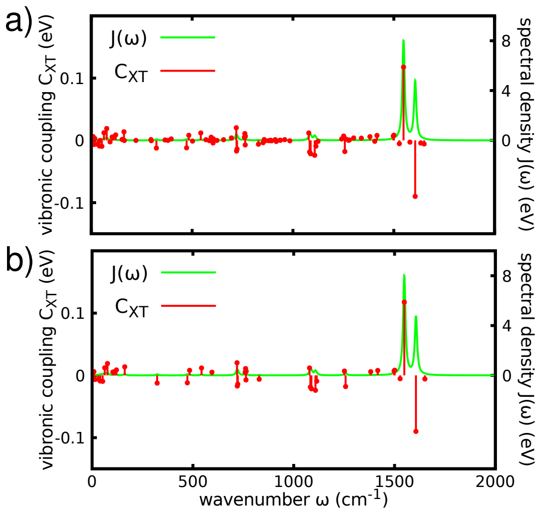
FIG. 3. Calculated vibronic couplings c_{XT} and spectral density J(\omega) for the bright S_2 state (of XT type) from excited-state gradients calculated at the TDDFT level for a (\text{OT4})_2 dimer. The local modes of a single OT4 fragment have been used for the determination of the vibronic couplings while keeping the other fragment frozen. a) Full normal mode vibronic couplings and corresponding spectral density obtained by convolution with a Lorentzian ( \Delta = 0.1\overline{\Delta\omega} ). b) Vibronic couplings above a threshold value of |c_{XT}| = 0.005 eV, and corresponding spectral density. By imposing this threshold, the full number of modes for each OT4 fragment is reduced from 84 to 39. The reorganisation energy changes only marginally, by 3%.
