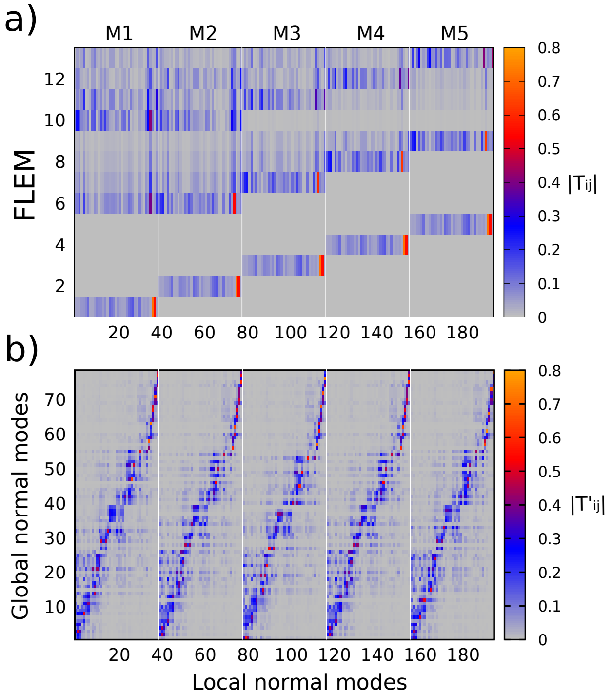
FIG. 5. Graphical representation of effective modes in the basis of the original local NMs. a) First layer effective mode (FLEM) space of dimension N_s = 13 in the band-diagonal representation. The absolute values of the transformation matrix elements T_{ij} , i = 1, \dots, N_s , j = 1, \dots, N_{\text{ph}} , according to Eq. (23) are shown. b) Truncated effective mode space for k=6 (truncation at the sixth order), leading to K = kN_s = 78 modes; the re-diagonalized representation is shown, i.e., global NMs of the truncated effective Hamiltonian. The graphical representation shows absolute values of the transformation matrix elements T'_{ij} , i = 1, \dots, kN_s , j = 1, \dots, N_{\text{ph}} , where the transformation \mathbf{T}' is a concatenation of Eq. (23) and the additional transformations of Eq. (29) and Eq. (30).
