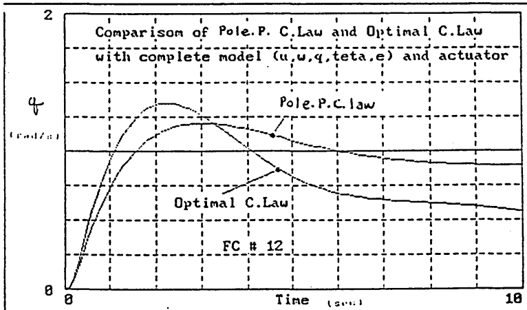
figure 3.13 - pitch-rate time response of both designs with the complete model of the aircraft and actuator at 10000 ft, mach 0.30
