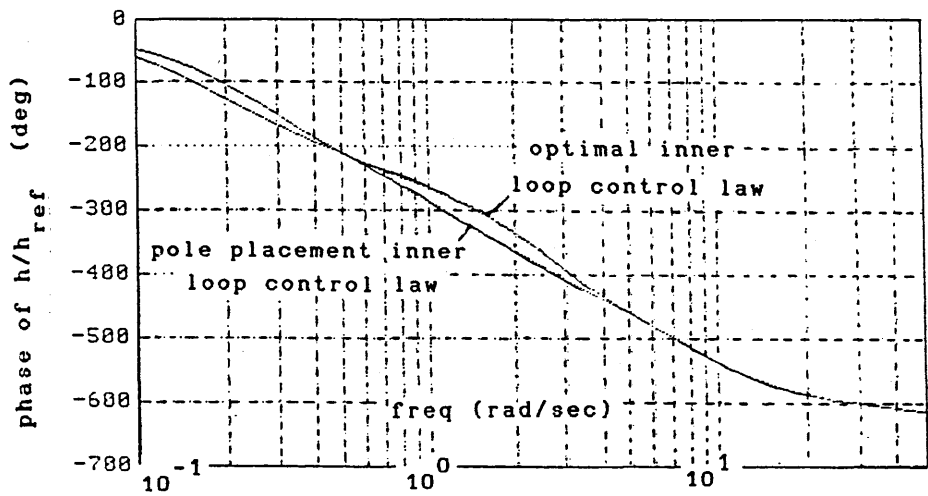
figure 8.5 - altitude frequency response of the autopilot at 20000 ft mach 0.70
