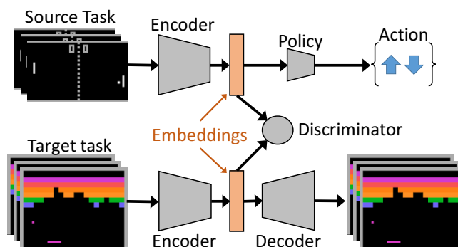
Figure 1: Our agent’s architecture for domain adaptation, combining adversarially discriminative domain adaptation and adversarial autoencoder architectures. A fully-trained source task is depicted on top, while on the bottom is the target task autoencoder.
