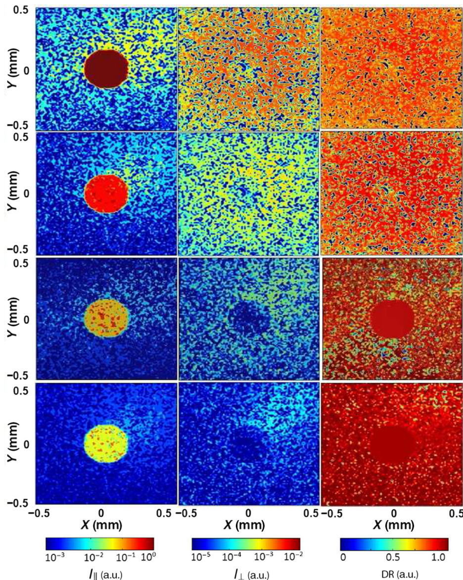
Fig. 8 Spatial intensity distributions of co- and cross-polarized light I_{\parallel,\perp}(x, y) and depolarization ratio \text{DR}(x, y) counted for the modeling media with optical properties corresponding to the phantom II (see Table 1). The roughness from top row to bottom correspond, respectively, to h_{\text{rms}} = 0, 2.5, 34.4, and 65.8 \mu\text{m} , and L_{\text{corr}} = 100 \mu\text{m} .
