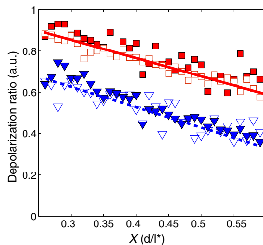
Fig. 11 Radial distribution of DR measured experimentally for the phantom I ( \square ) and II ( \nabla ) in comparison with the results obtained by the electric field MC ( \blacksquare and \blacktriangledown ). The solid and dashed lines represent the linear fits. The standard deviation for the results of experimental studies is in a range of 5–7%.
