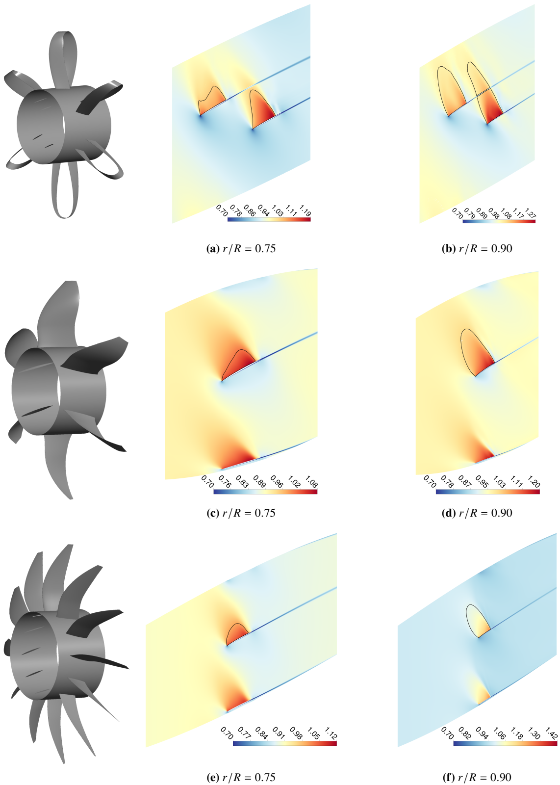
Fig. 6 Mach number at the 75% and 90% radial positions for the Boxprop, 6-bladed, and 12-bladed conventional propellers. The black lines denote regions of Mach equal to unity.
