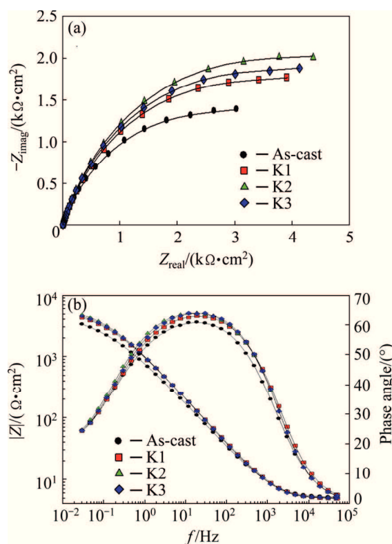
Fig. 2 Nyquist (a) and Bode (b) plots for CuAlNi alloy in 0.9% NaCl solution
