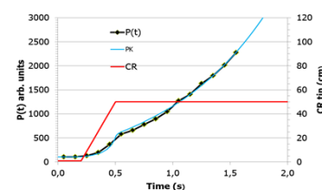
MCNP5/SCF: Ejection of the central pin
