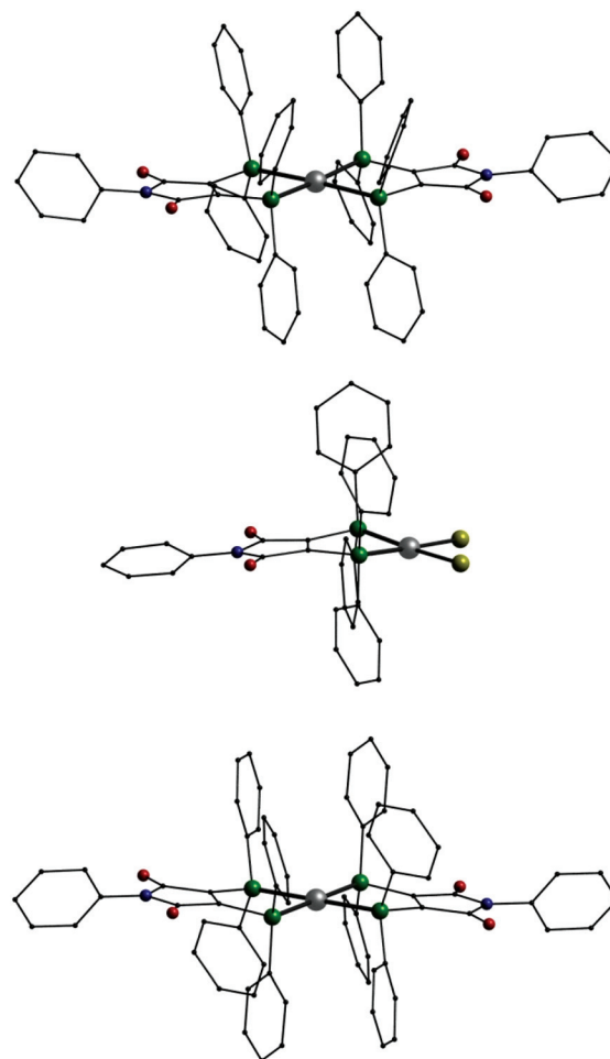
Fig. 7 Molecular structures of [\text{Pd}(\text{L1}')_2] ( 11 , top), [\text{PdCl}_2(\text{L1})] ( 12 , middle) and the dication [\text{Pd}(\text{L1})_2]^{2+} in 13 (bottom); Pd: grey, P: green, Cl: yellow, O: red, N: blue, C: black, H atoms omitted.
