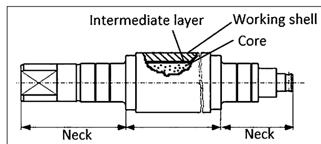
Figure 1 Roller cross section [7]
