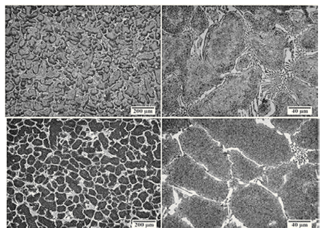
Figure 3 Microstructure of working shell of HCS rolls. Before heat treatment (above), after heat treatment (bellow)
