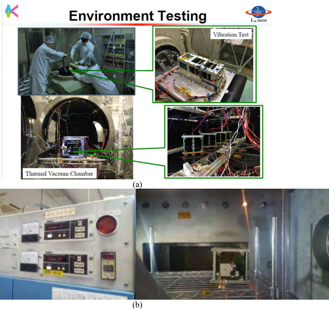
FIGURE 8. a) Launch conditions: vibration test b) environment conditions: vacuum test and thermal vacuum test.
