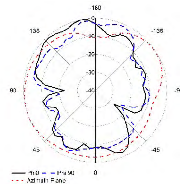
FIGURE 6. 2D measured radiation pattern of the antenna.
