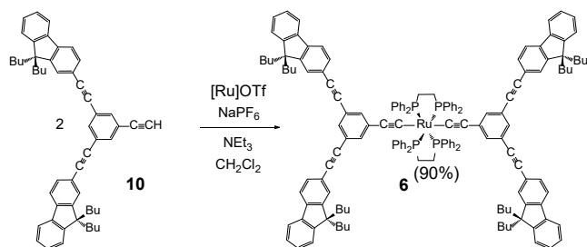
Scheme 2. Synthesis of the Ru(II) Complex 6 .
