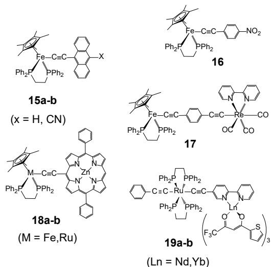
Chart 4. Selected Examples of Redox-switchable Lumino-phores.
