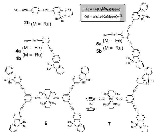
Chart 2. Target 2-Fluorenyl-based Alkynyl Complexes.
