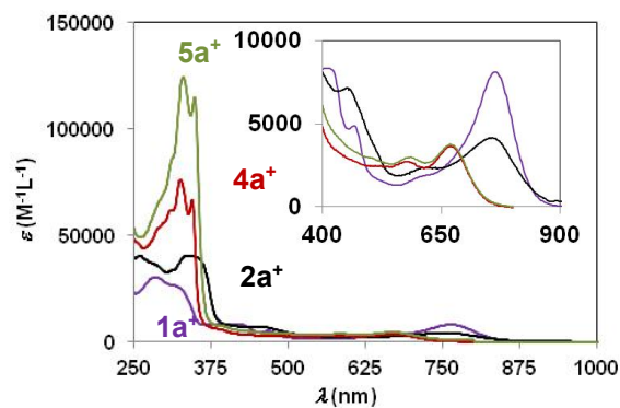
Figure 3. UV-Vis-Near IR absorption spectra for 1a[PF 6 ] , 2a[PF 6 ] , 4a[PF 6 ] and 5a[PF 6 ] in CH 2 Cl 2 at 25 °C.
