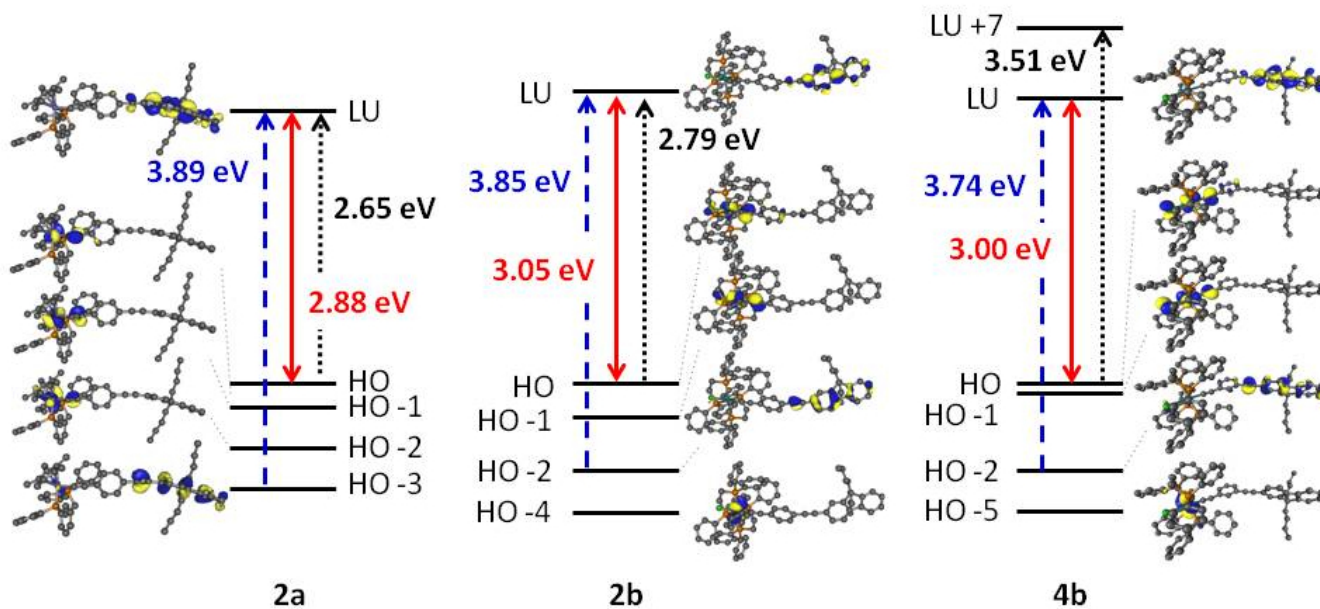
Figure 8. Selected metallic and fluorenyl-based Kohn-Sham frontier molecular orbitals for 2a , 2b and 4b illustrating the HOMO-LUMO gap (red arrows). The first MLCT and LC transitions are indicated by dark arrows and dashed blue arrows, respectively. Hydrogen atoms are omitted for clarity.
