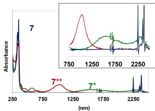
Figure 5. Spectroelectrochemistry in the near UV-Vis-near-IR range for complex 7 in CH 2 Cl 2 (0.2 M TBAH) at -30 °C. Inset: expansion of the 750-2500 nm region.
