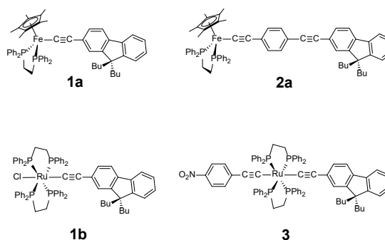
Chart 1. Extant 2-Fluorenyl-based Alkynyl Complexes.
