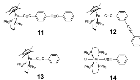
Chart 3. Selected Alkynyl Complexes used as References.
