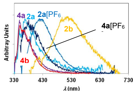
Figure 6. UV-Vis emission spectra for 2a-b , 4a-b , 2a [PF 6 ] and 4a [PF 6 ] complexes in dichloromethane at 300 K.
