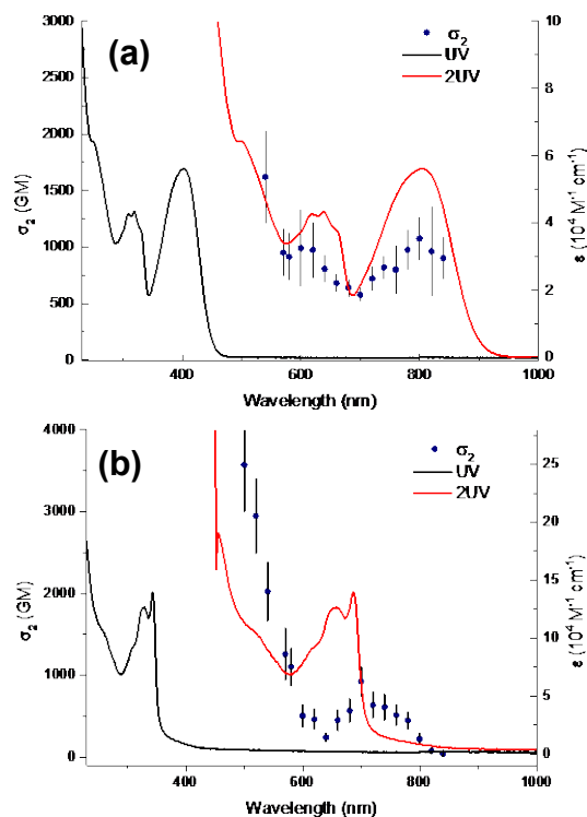
Figure 7. Apparent two-photon absorption cross-sections (in Göppert-Mayer units) for 2b (a) and 4b (b) in dichloromethane at 25 °C by open-aperture Z-scan measurements. The 2PA spectral data are overlaid by the one-photon absorption spectrum (black) and the one-photon absorption spectrum plotted at 2\lambda (red).
