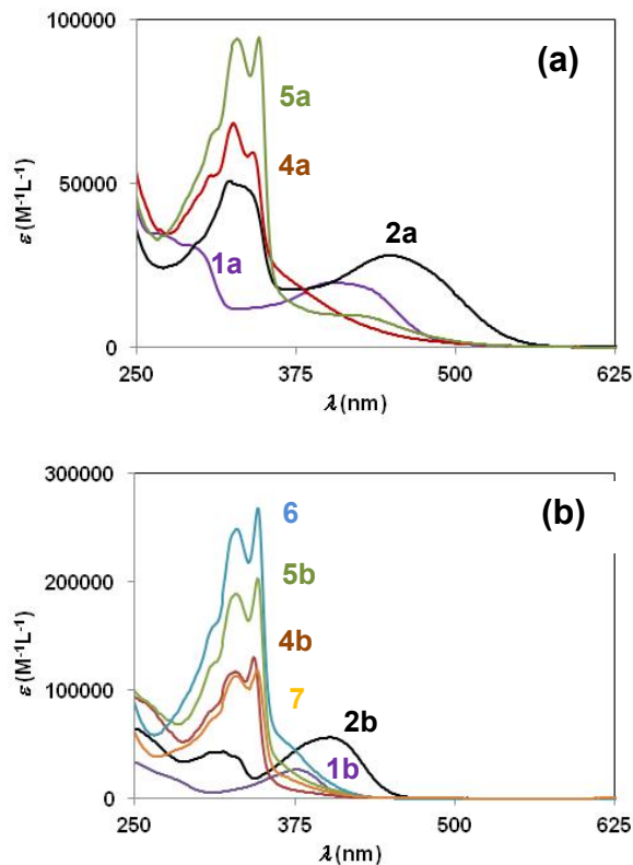
Figure 2. UV-Vis-Near IR absorption spectra for (a) 1a , 2a , 4a and 5a and (b) 1b , 2b , 4b , 5b and 6 complexes in CH 2 Cl 2 at 25 °C.
