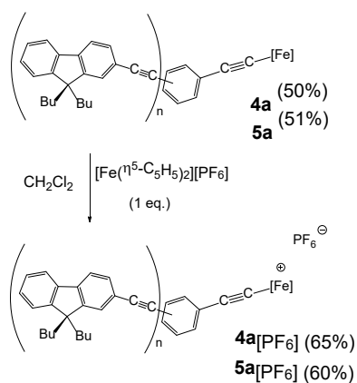
Scheme 4. Synthesis of the Fe(III) Complexes 4a [PF 6 ] and 5a [PF 6 ] ([Fe] = Fe( \eta^5 -C 5 Me 5 )( \kappa^2 -dppe)).
