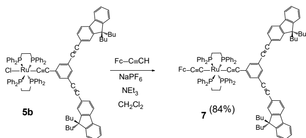
Scheme 3. Synthesis of the Ru(II) Complex 7 .
