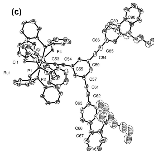
Figure 1. ORTEP representations of 2b (a), 4b (b) and 5b (c) at the 50% probability level. Selected distances (Å) and angles (deg): (a) Ru1-C11 2.4953(11), Ru1-P1 2.3472(14), Ru1-P2 2.3739(11), Ru1-P3 2.3806(11), Ru1-P4 2.3592(14), Ru1-C53 2.002(4), C53-C54 1.205(5), C54-C55 1.426(5), C61-C62 1.201(6), C66-C67 1.467(6), P1-Ru1-P2 82.34(4), P3-Ru1-P4 81.85(4), C11-Ru1-C53 178.79(10), Ru1-C53-C54 175.8(3), C53-C54-C55 174.9(5), C58-C61-C62 177.5(6), C61-C62-C63 178.5(6), C57-C58-C63-C64 167.4; (b) Ru1-C11 2.4522(9), Ru1-P1 2.3436(9), Ru1-P2 2.3453(10), Ru1-P3 2.3943(10), Ru1-P4 2.4063(9), Ru1-C53 1.996(2), C53-C54 1.214(3), C54-C55 1.438(3), C61-C62 1.197(3), C66-C67 1.467(3), P1-Ru1-P2 82.06(4), P3-Ru1-P4 81.82(4), C11-Ru1-C53 175.97(5), Ru1-C53-C54 178.20(17), C53-C54-C55 168.1(2), C59-C61-C62 175.9(2), C61-C62-C63 174.6(2), C58-C59-C63-C64 59.1; (c) Ru1-C11 2.5013(14), Ru1-P1 2.3713(13), Ru1-P2 2.3954(12), Ru1-P3 2.3693(12), Ru1-P4 2.3463(14), Ru1-C53 1.994(5), C53-C54 1.224(6), C54-C55 1.417(6), C61-C62 1.169(7), C66-C67 1.457(8), C84-C85 1.200(7), C89-C90 1.479(7), P1-Ru1-P2 81.17(5), P3-Ru1-P4 81.64(5), C11-Ru1-C53 176.87(13), Ru1-C53-C54 176.9(4), C53-C54-C55 166.4(5), C58-C61-C62 177.8(6), C61-C62-C63 174.5(6), C57-C58-C63-C64 16.0, C59-C84-C85 177.5(6), C84-C85-C86, C58-C59-C86-C87 -131.5.
