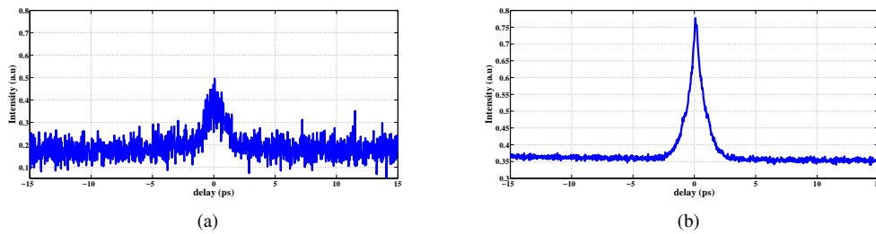
Fig. 6. Measured pulse from autocorrelator at the output of: (a) FSO 1, and (b) AORF Mamyshev regeneration.
