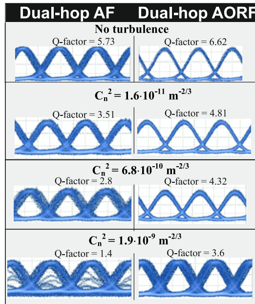
Fig. 11. Measured eye-diagrams for dual-hop FSO link with AF and AORF with and without turbulence.
