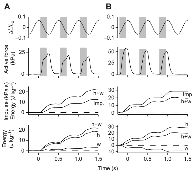
Fig. 3. Example recordings. Net positive work (A) and net negative work (B) for a peroneus longus (PL) fibre bundle (blotted mass, 13.37 mg; L_0 , 11.5 mm). Three cycles of sinusoidal movement at 2 Hz and peak-to-peak amplitude 1.5 mm ( \approx 13.0\% L_0 ), stimulus duty cycle 0.3 and stimulus phase +0.1 in A and -0.4 in B. \Delta L/L_0 is length change expressed as a fraction of L_0 , the length giving maximum isometric force. Active force is expressed relative to cross-sectional area. The shading indicates the period of stimulation. Impulse is the integral of active force and time ( \text{kPa s} ). Three forms of energy ( \text{J kg}^{-1} muscle fibre) are shown: h, cumulative heat output; w, cumulative net work, where net work is the sum of positive and negative work; and h+w, the cumulative sum of heat output and net work. h+w is a measure of cost and is included in the graph with impulse to ease comparison of the results shown in A and B.
