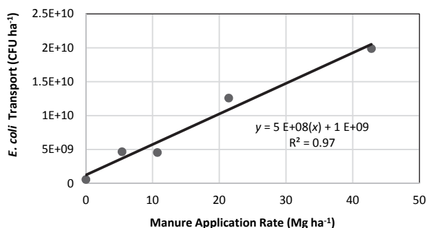
Figure 3. E. coli transport as affected by manure application rate.
