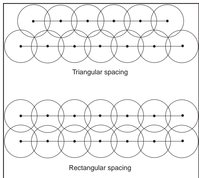
Figure 1. Effect of sprinkler spacing and arrangement. Note that the rectangular pattern requires closer spacing to achieve full coverage and reasonable uniformity.
