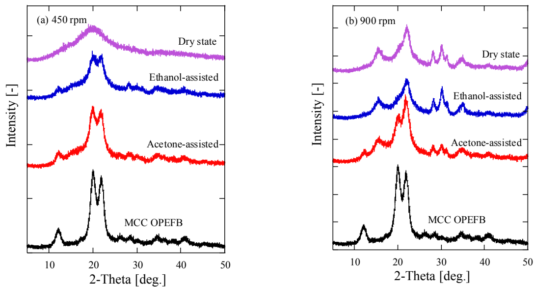
Figure 1. The XRD patterns (a) mechanical grinding with 450 rpm and 4 h; (b) 900 rpm and 30 min
