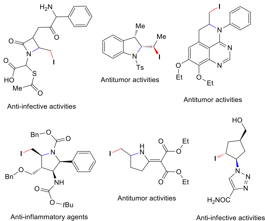
Figure 1. Selected bioactive vicinal iodoamine derivatives
