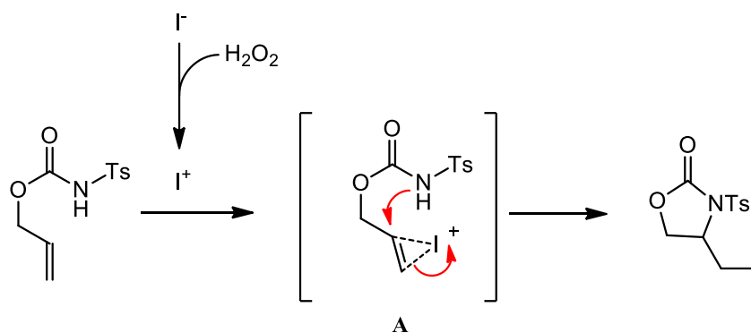
Scheme 4. Proposed iodoamination reaction mechanism
