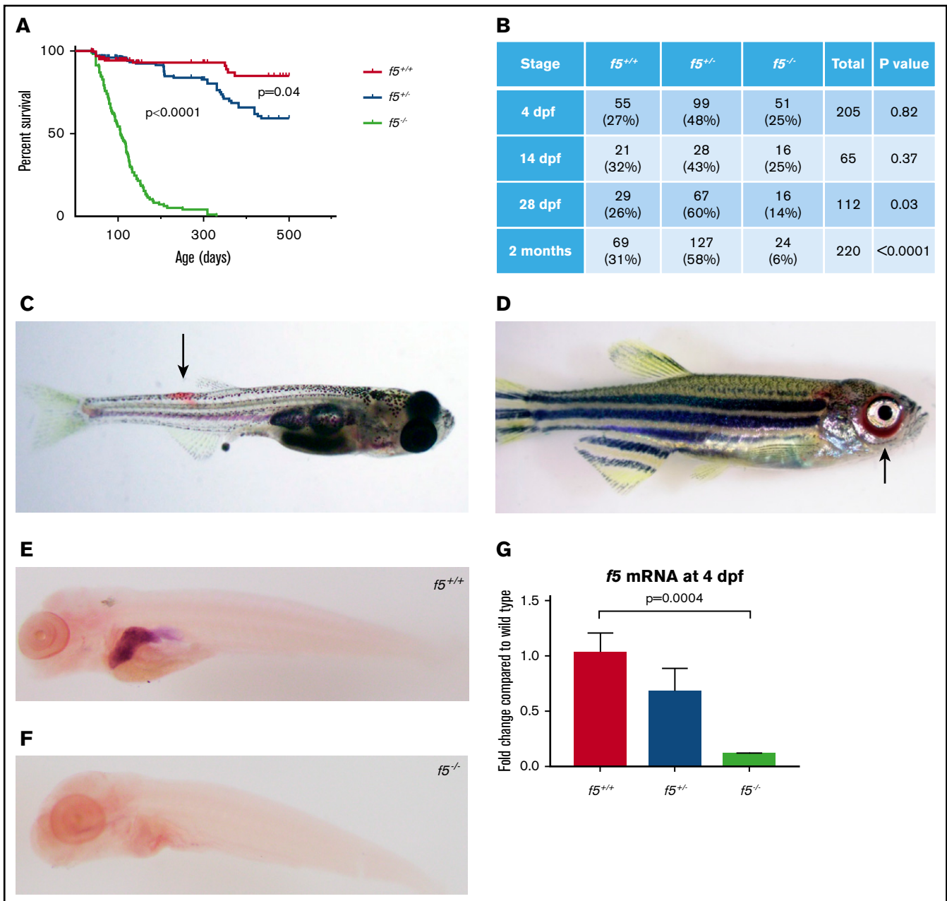
Figure 2. Phenotypes of f5 homozygous mutants reveal adult lethality and spontaneous hemorrhage in homozygous mutant adult fish. (A) Survival curves of zebrafish offspring from f5 +/- incrosses, starting at 2 months of age, demonstrate progressive loss of 90% of homozygotes by 7 mpf. Heterozygotes also demonstrate statistically significant decreased survival compared with wild-type fish, with 50% mortality by 1.5 years of age. (B) Genotype distributions of offspring from f5 +/- incrosses evaluated at various stages demonstrate loss of homozygotes beginning at 28 dpf. (C) Spontaneous hemorrhage distal to the dorsal fin (arrow) in a 4-week-old homozygous mutant fish. (D) Severe spontaneous periorbital hemorrhage (arrow) grossly visible in a 5-week-old homozygous mutant fish just before death. Similar bleeding was not observed by blinded observers in heterozygous or wild-type clutchmates. Whole mount in situ hybridization with an antisense probe demonstrates localization of f5 expression to the liver in f5 +/+ zebrafish at 5 dpf (E), but not in f5 -/- mutants (F). (G) Total mRNA was prepared from pooled larvae (4 dpf, n = 21 for each genotype) followed by quantitative real-time PCR. Error bars represent standard deviation and statistical significance was determined by a Student t test.
