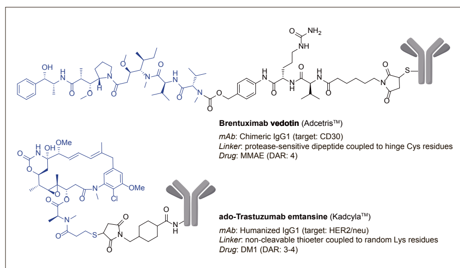
Fig. 3. Schematic representation of the structure of Adcetris TM and Kadcyla TM . In the first case, monomethyl auristatin E (MMAE), equipped with a cleavable linker, is coupled to the cysteine residues of an anti-CD30 chimeric antibody. In the second case, the potent maytansinoid DM1 is coupled to primary amino groups of the humanized anti-HER2 antibody trastuzumab using a stable linker.
