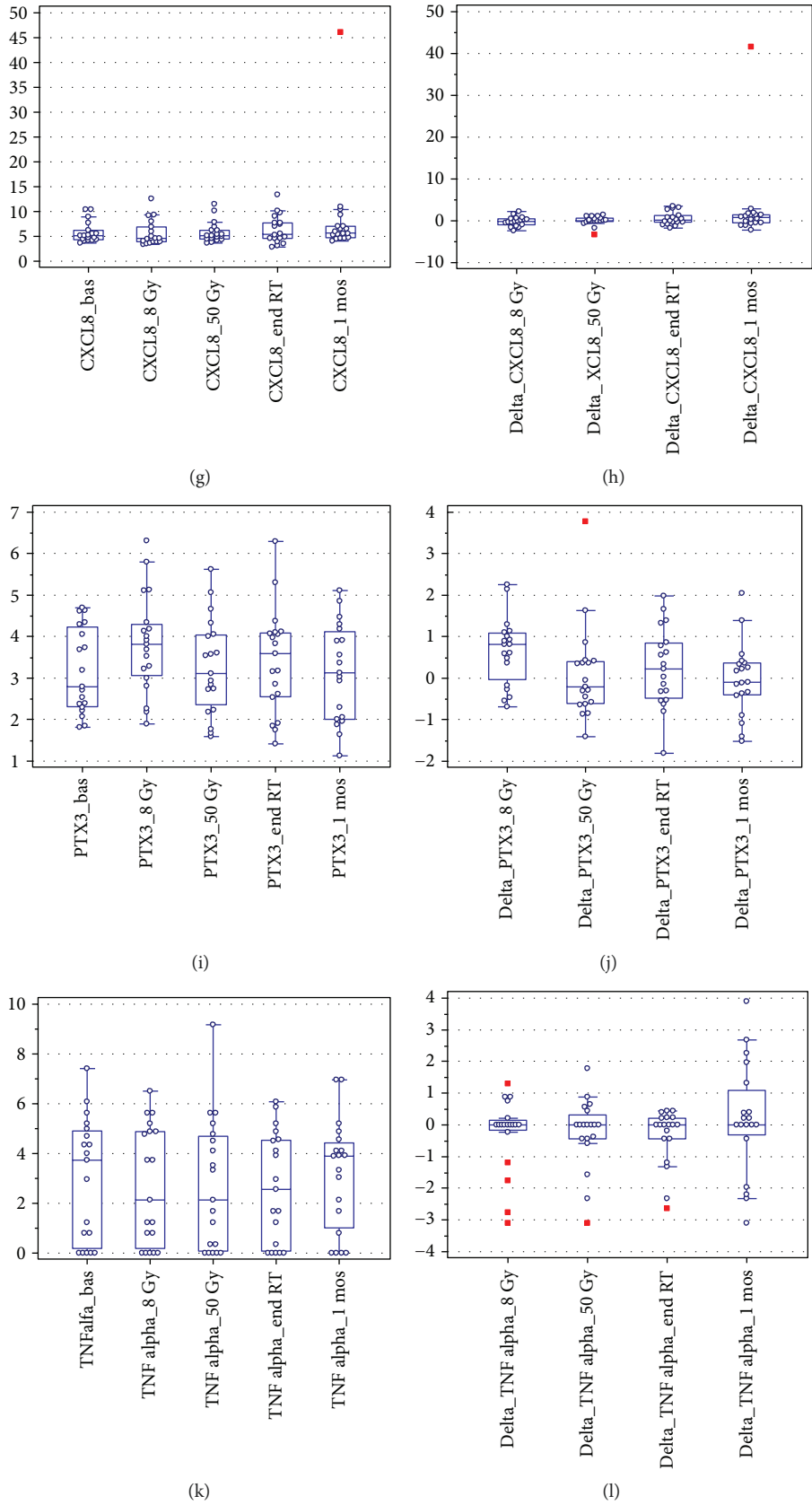
FIGURE 1: Plasma levels of the selected inflammatory molecules for all measurement points: absolute values (a, c, e, g, i, and k) and absolute variations with respect to baseline (b, d, f, h, j, and l). 1 mos: 1 month; RT: radiotherapy. Units of measure are pg/ml for IL-1b, IL-6, CXCL8, CCL2, and TNF alpha; ng/ml: PTX3.
