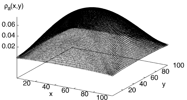
FIG. 2. Local density of active sites \langle \rho_a(x, y) \rangle , in the case of boundary dissipation; the linear lattice size is L = 100 , and h = 10^{-4} .
