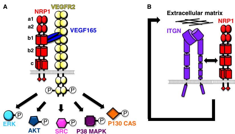
Figure 1. NRP1-regulated signaling pathways in endothelial cells in vitro . (A) VEGF165 induces complex formation between NRP1 and VEGFR2 to enhance VEGFR2 signaling in endothelial cells in vitro . In particular, biochemical studies suggested possible roles for NRP1 in the VEGF-mediated induction of pathways involving the activation of ERK, AKT, SRC, P38 MAPK, and p130 CAS. (B) NRP1 regulates integrin-dependent fibronectin remodeling in primary arterial endothelial cells and tumor cells in a mechanism that depends on the NRP1 cytoplasmic domain, but is thought to be VEGFR2 independent.
