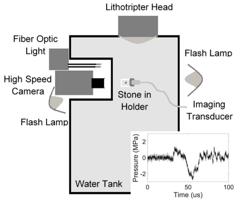
Figure 1. Experimental arrangement to visualize crevice bubbles on the kidney stone surface by expanding them with a lithotripter pulse. Stones were placed pre-focal and off axis and were visualized with a high-speed camera and ultrasound transducer when the lithotripter pulse (inset) arrived.
