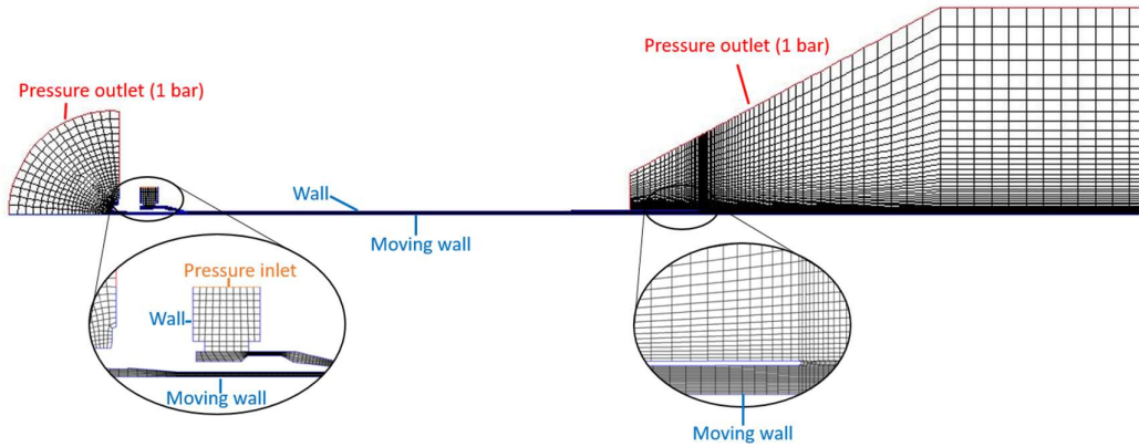
Figure 2: Mesh of the flow domain and its boundary conditions.
