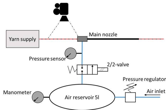
Figure 1: Sketch of the experimental setup.
