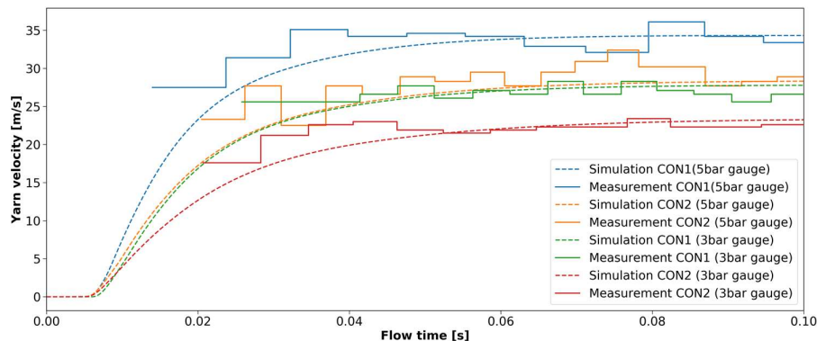
Figure 4: Experimental and simulated yarn velocity for a polymer coated yarn.
