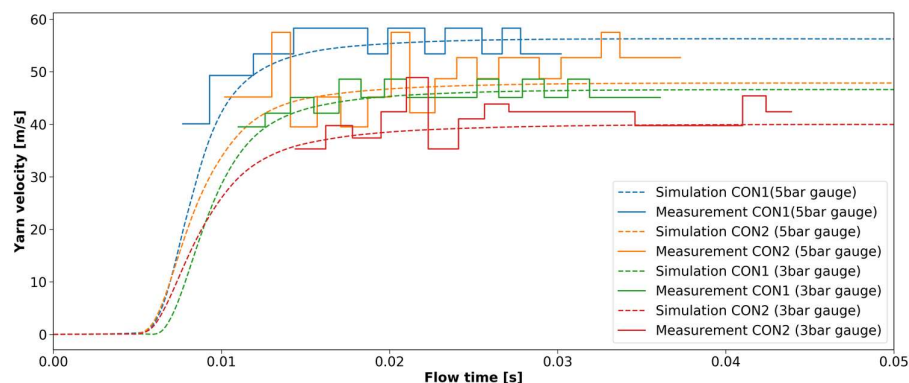
Figure 5: Experimental and simulated yarn velocity for a cotton yarn.
