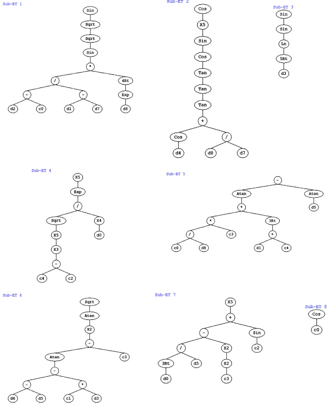
Fig. 4. GEP model expression tree for I-H steel beams.
