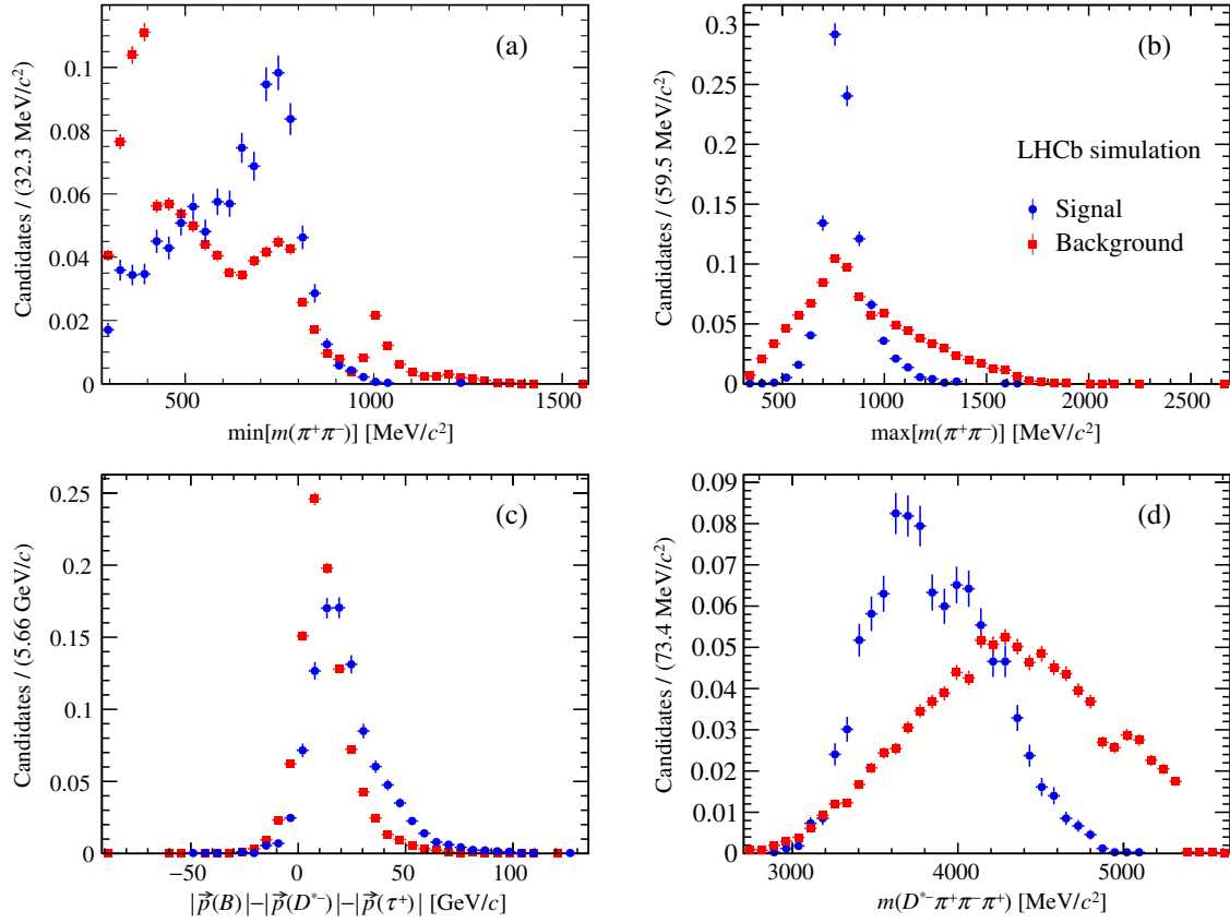
FIG. 10. Normalized distributions of (a) \min[m(\pi^+\pi^-)] , (b) \max[m(\pi^+\pi^-)] , (c) approximated neutrino momentum reconstructed in the signal hypothesis, and (d) the D^{*-}3\pi mass in simulated samples.
