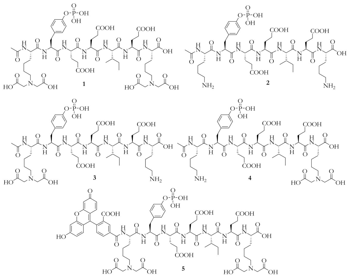
Figure 1. Chemical structures of peptides 1–4 containing 0–2 IDA groups and fluorescein-labelled peptide derivative 5 .
