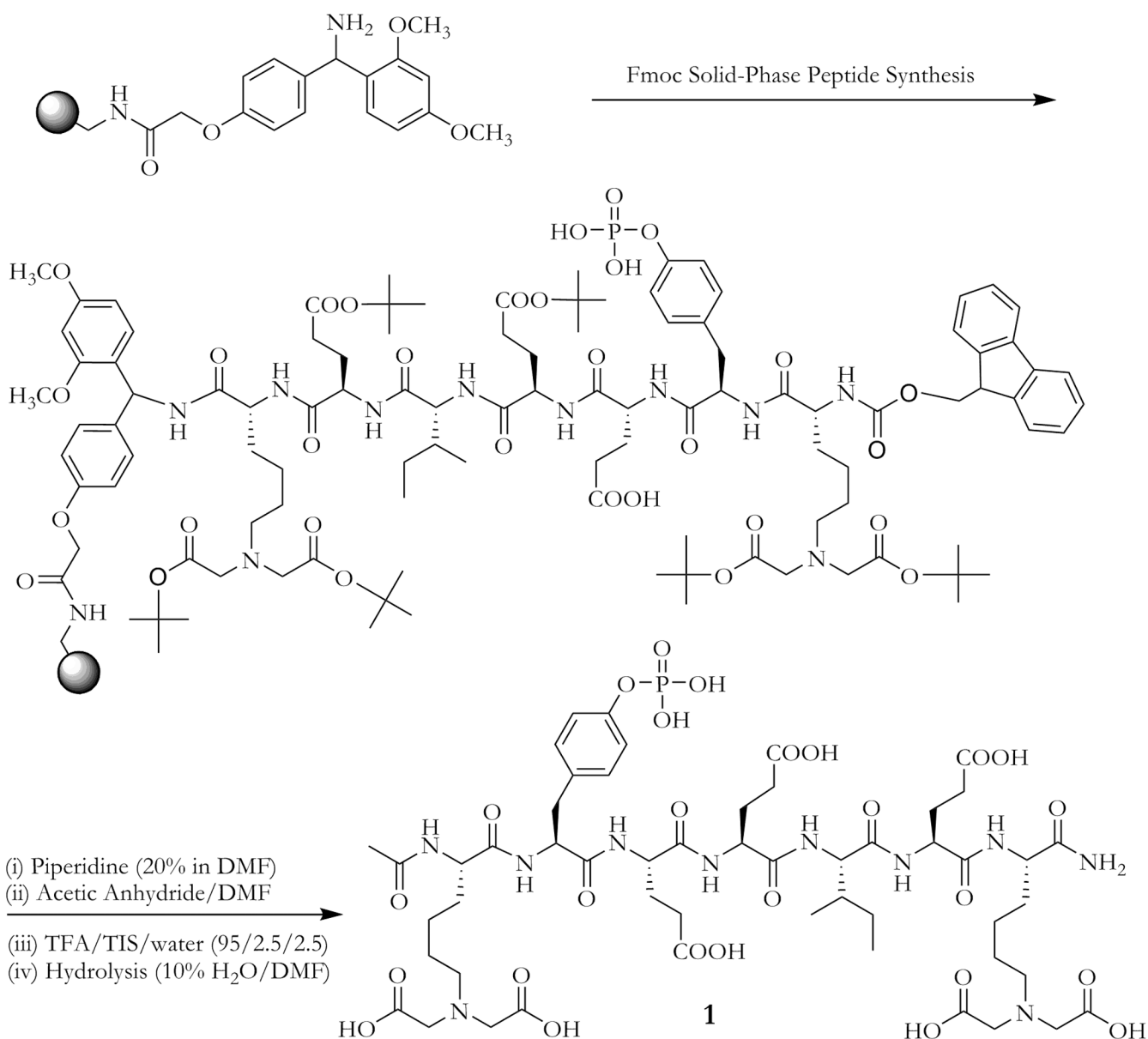
Scheme 1. Solid-phase synthesis of peptide 1 .
