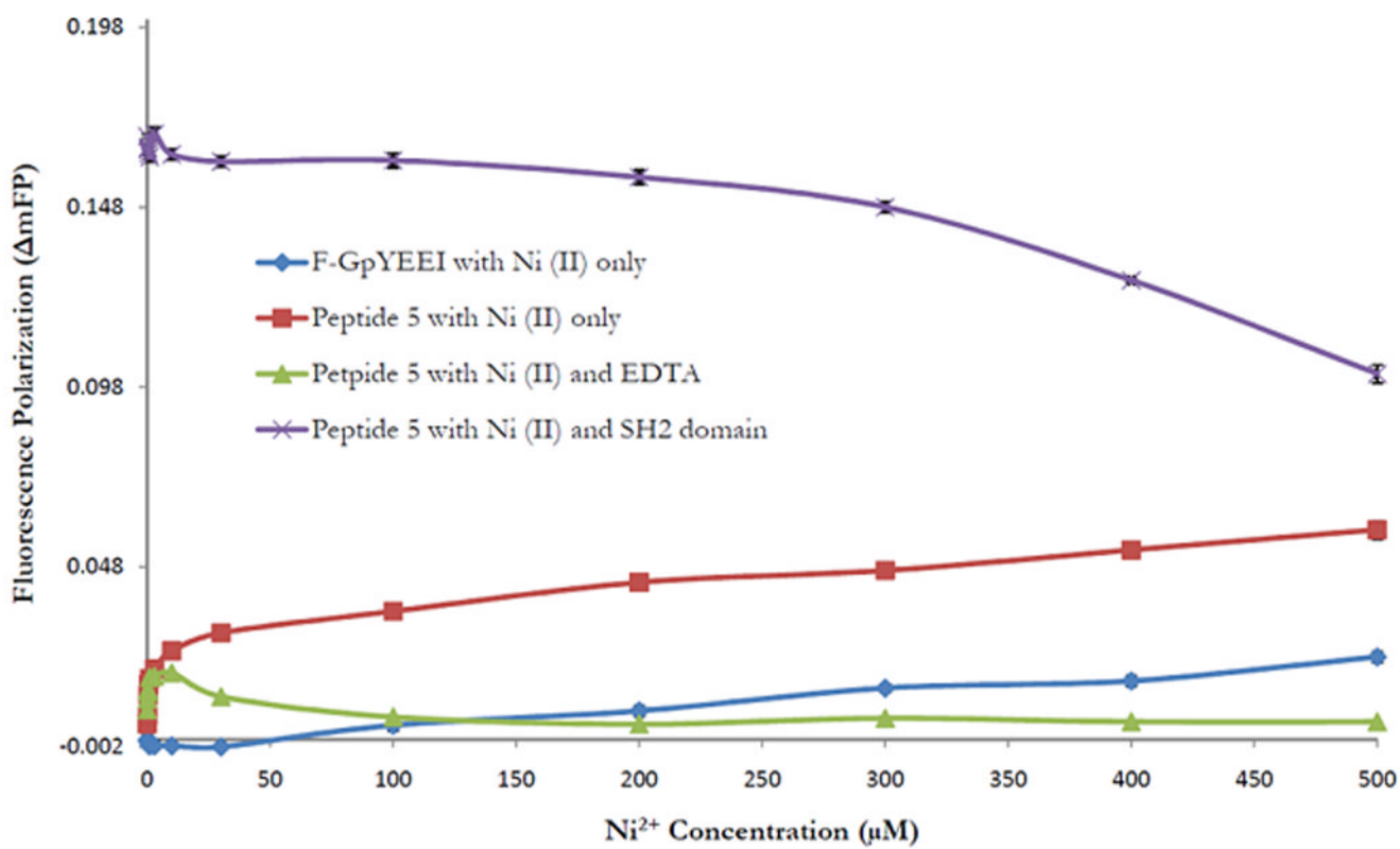
Figure 3. The fluorescence polarization values in different saturation assay conditions.
