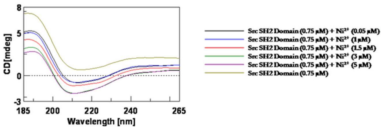
Figure 5. The CD spectra of different concentration of \text{Ni}^{2+} and fixed concentration of Src SH2 domain.
