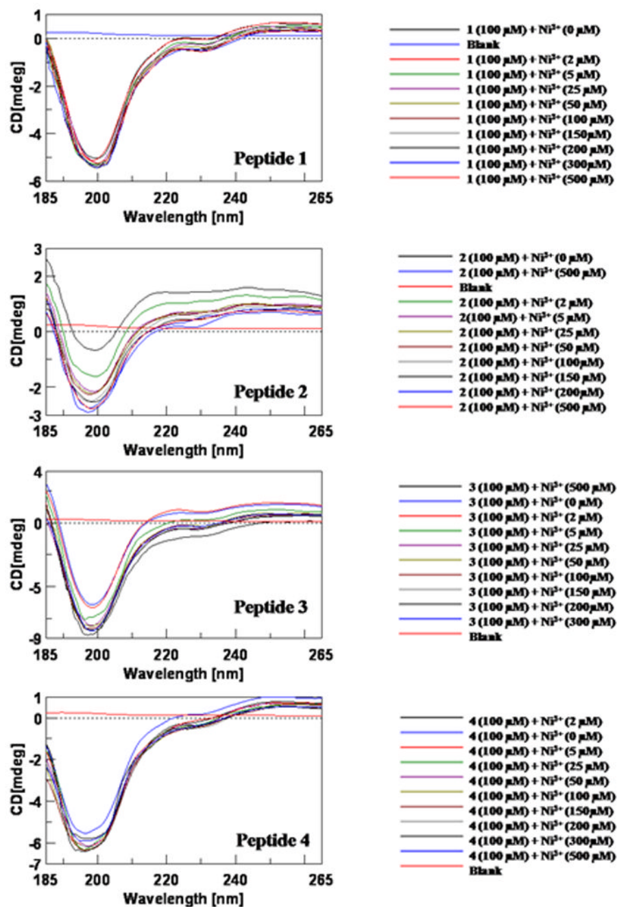
Figure 4. The CD spectra of peptides 1–4 (100 \mu\text{M} ) in the presence of different concentrations of \text{Ni}^{2+} in the absence of the Src SH2 domain.
