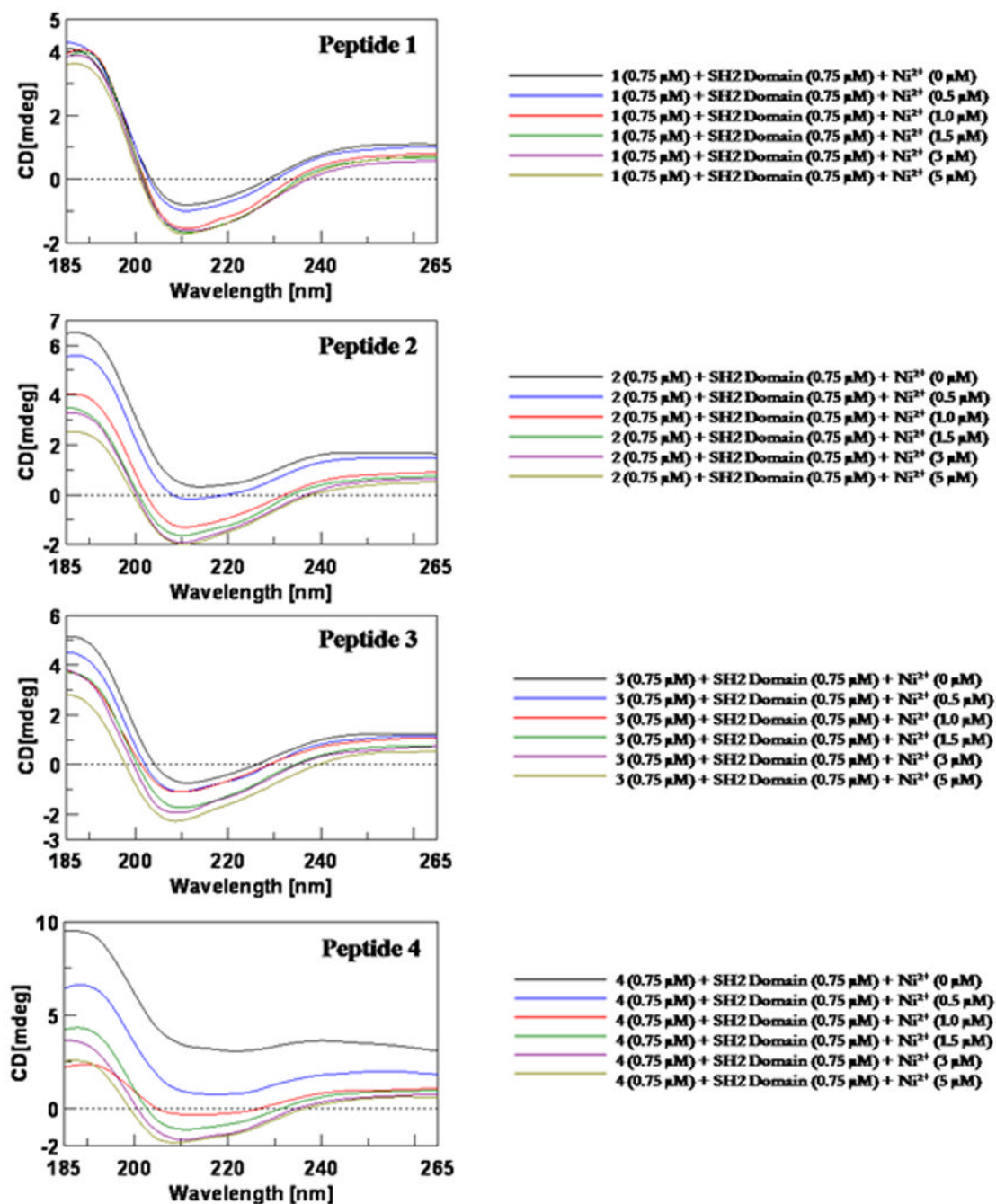
Figure 6. The CD spectra of fixed concentration of peptides 1–4 and the Src SH2 domain with different concentrations of \text{Ni}^{2+} .
