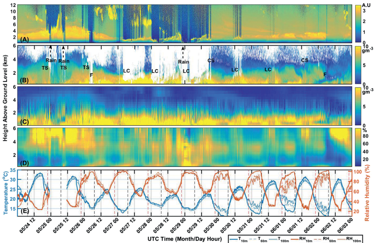
FIG. 10. (a) DIAL relative backscatter in aerosol units and (b) absolute humidity at the Orange Grove site (highlighting aerosol and cloud structures up to 12 km by NCAR); (c) AERI absolute humidity at the lower Orange Grove site (by UO); (d) MWR relative humidity (George site; outside the valley by UND); (e) relative humidity and temperature at different levels from the 100-m tower (mast 25) near DIAL and AERI. In (e), black dashed line indicates sunrise, and the orange line indicates sunset. Low clouds (LC); clear skies (CS); fog (F); thunderstorms (TS). Rain events are also indicated.
