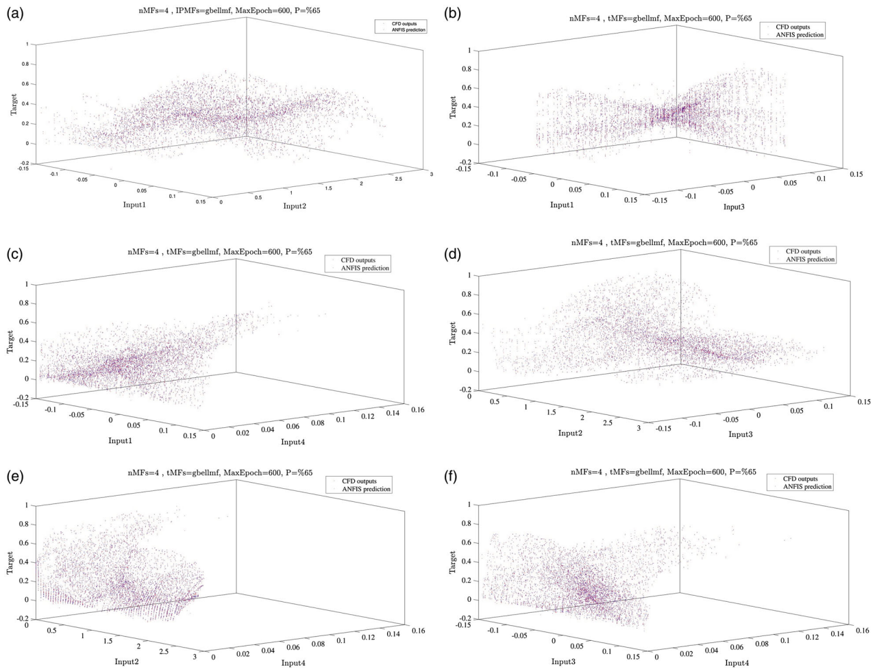
Figure 7. (a) Compare CFD output and ANFIS method prediction using inputs 1 and 2. (b) Compare CFD output and ANFIS method prediction using inputs 1 and 3. (c) Compare CFD output and ANFIS method prediction using inputs 1 and 4. (d) Compare CFD output and ANFIS method prediction using inputs 2 and 3. (e) Compare CFD output and ANFIS method prediction using inputs 2 and 4. (f) Compare CFD output and ANFIS method prediction using inputs 3 and 4.
