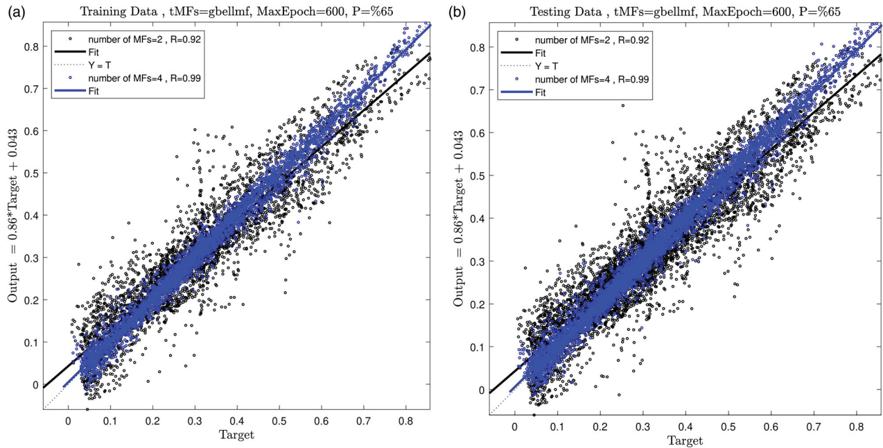
Figure 5. (a) Training with using three inputs and different number of MFs (ANFIS method). (b) Testing with using three inputs and different number of MFs (ANFIS method).
