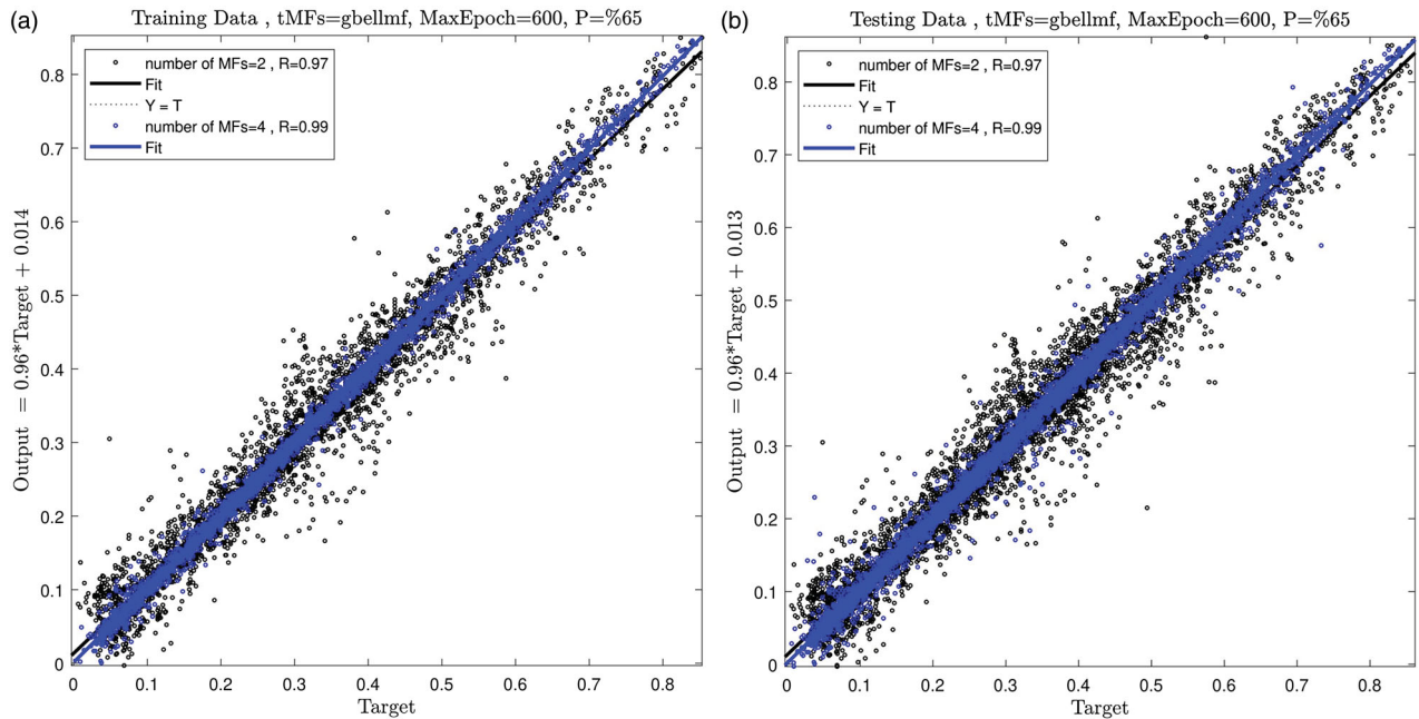
Figure 6. (a) Training with using four inputs and different number of MFs (ANFIS method). (b) Testing with using four inputs and different number of MFs (ANFIS method).
