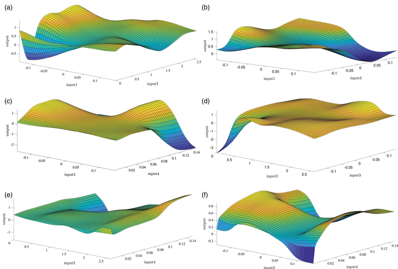
Figure 9. (a) Output prediction in Full intelligence of ANFIS method using inputs 1 and 2. (b) Output prediction in Full intelligence of ANFIS method using inputs 1 and 3. (c) Output prediction in Full intelligence of ANFIS method using inputs 1 and 4. (d) Output prediction in Full intelligence of ANFIS method using inputs 2 and 3. (e) Output prediction in Full intelligence of ANFIS method using inputs 2 and 4. (f) Output prediction in Full intelligence of A.
