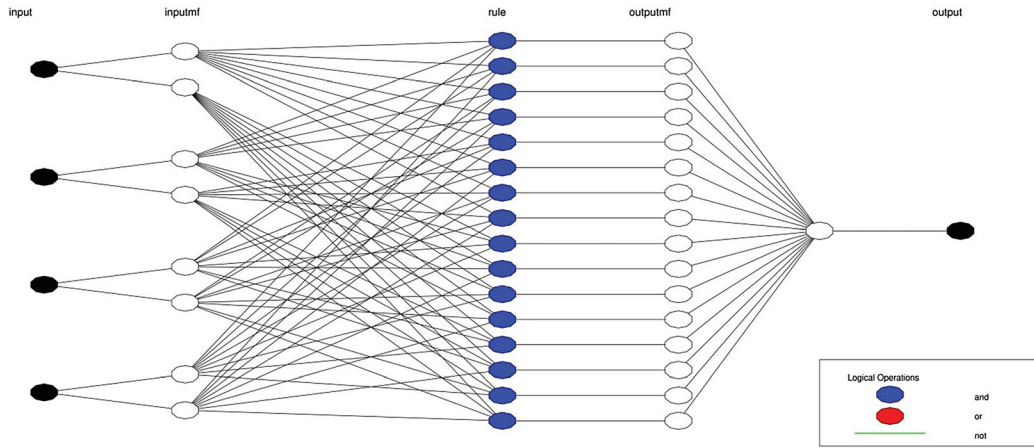
Figure 1. Schematic of the ANFIS structure.
