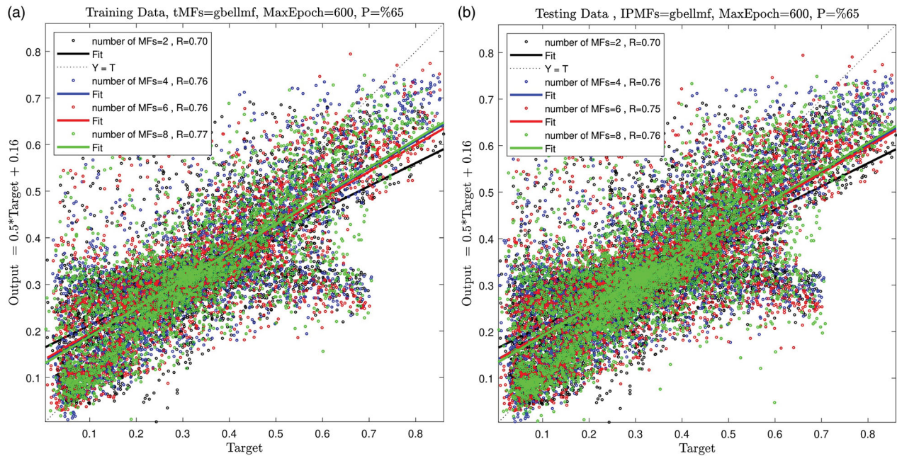
Figure 3. (a) Training with using two inputs and different number of MFs (ANFIS method). (b) Testing with using two inputs and different number of MFs (ANFIS method).
