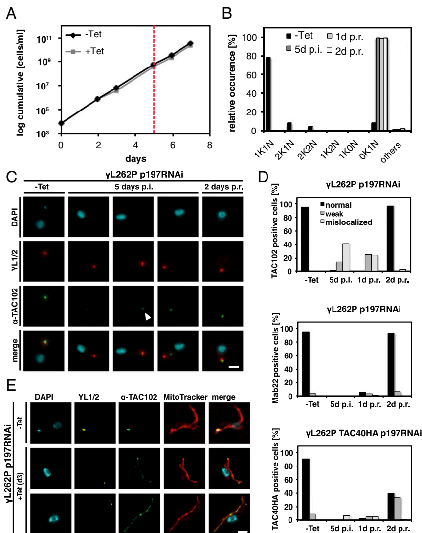
Fig. 5. TAC biogenesis after recovery from p197 depletion. (A) Growth curve of \gamma L262P p197 RNAi cells. After 5 d of p197 RNAi induction, cells were washed and grown in medium without Tet (red line). (B) Percentage of cells with kDNA and nucleus in p197 RNAi induced and uninduced trypanosomes ( n \sim 100 ). (C) TAC102 (green), YL1/2 (basal body, red), and DAPI (DNA, cyan) stained cells after 0 and 5 d of Tet induction (postinduction, p.i.) and 2 d postrecovery (p.r.) are shown. White arrowhead points to an example for a weak signal. (D) Quantitative analysis of TAC102 ( n = 106 ), Mab22 ( n \geq 93 ), or TAC40HA ( n \geq 119 ) in uninduced (–Tet), 5 d-induced (5 d p.i.), and 1 or 2 d after removing Tet (1 d p.r., 2 d p.r.) in \gamma L262P p197 RNAi cells. As a control for the staining, only cells with a discernible basal body signal were used. A black bar indicates a correct localized signal; a gray bar indicates a weak signal and a light gray a mislocalized signal. (E) p197 RNAi \gamma L262P cells were Tet induced for 3 d and stained with MitoTracker (mitochondrion, red), TAC102 (green), YL1/2 (basal body, yellow), and DAPI (DNA, cyan). (Scale bar: 2 \mu m).
