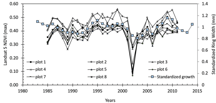
Fig. 9. Standardized ring width of B. papyrifera as a function of Landsat maximum-value NDVI observed in adjacent plots in Niobrara River Valley between 1985 and 2011. Missing points are due to cloud cover.
