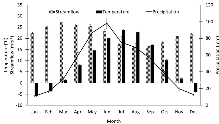
Fig. 3. Long-term average monthly streamflow of the Niobrara River ( m^3 \cdot s^{-1} ), air temperature ( ^{\circ}C ), and precipitation (mm) between 1950 and 2014.
