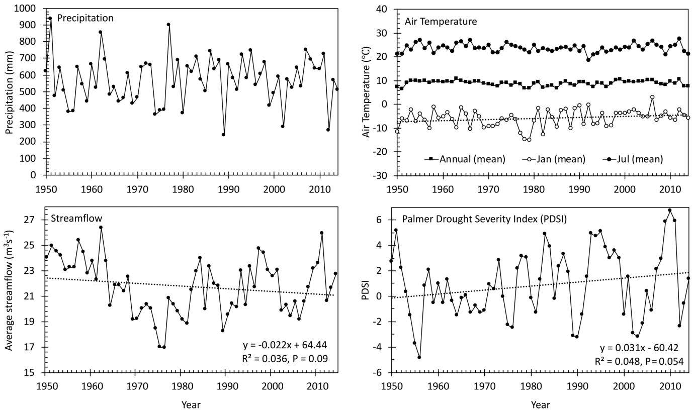
Fig. 3. Long-term average monthly streamflow of the Niobrara River ( m^3 \cdot s^{-1} ), air temperature ( ^{\circ}C ), and precipitation (mm) between 1950 and 2014.
