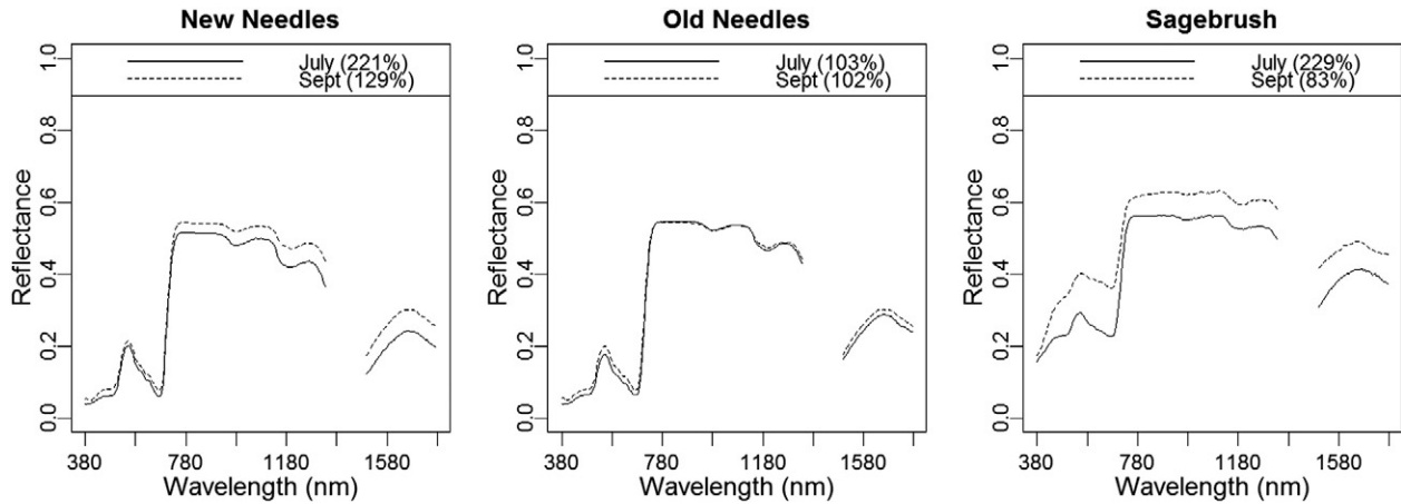
Fig. 5. Reflectance spectra on two observation dates in July and September for new needles, old needles, and sagebrush leaves. The values in the parentheses indicate LPMC.
