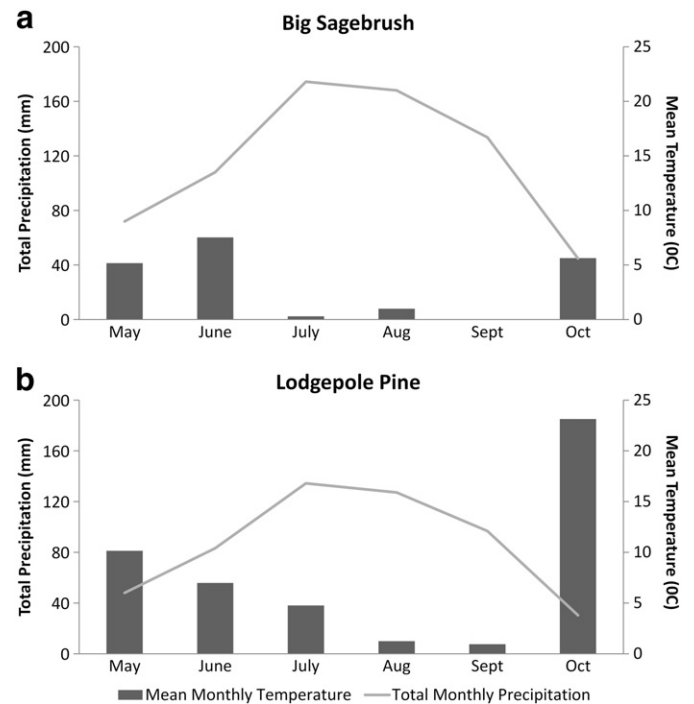
Fig. 1. 2012 climographs for weather stations proximate to sagebrush (a) and lodgepole pine (b) sites. Precipitation for (a) was measured at a station an average of 4 km north of the two sagebrush sampling sites, while temperature for (a) was measured at a station 500 m higher in elevation and 7 km to the south of the sampling sites. Precipitation and temperature (b) were measured at lodgepole pine site 2, approximately 12 km to the south of the lodgepole pine site 1. ( http://www.ncdc.noaa.gov/cdo-web/ , last accessed on May 30, 2014).
