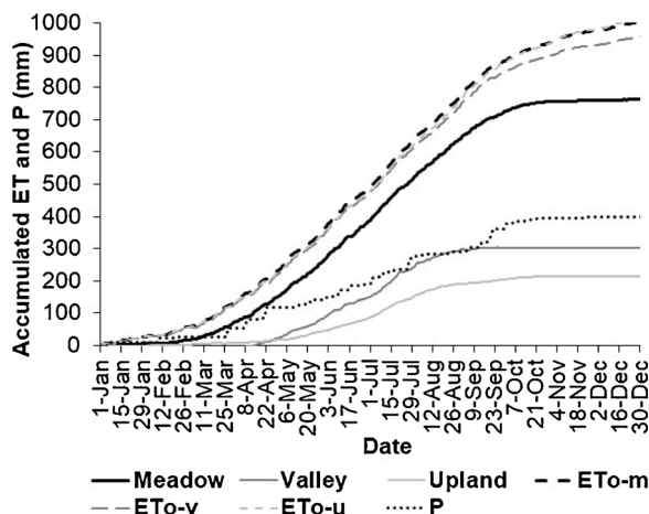
Fig. 2. Cumulative Reference Evapotranspiration at the Subirrigated Meadow ( ETo-m ), Dry Valley ( ETo-v ), and the Upland Dune ( ETo-u ), Precipitation ( P ) from the Automated Weather Data Network (AWDN) station, and Actual Evapotranspiration ( ET ) at the Subirrigated Meadow, Dry Valley, and Upland Dune sites within the Gudmundsen Sand Hills Laboratory, Nebraska in 2004.
