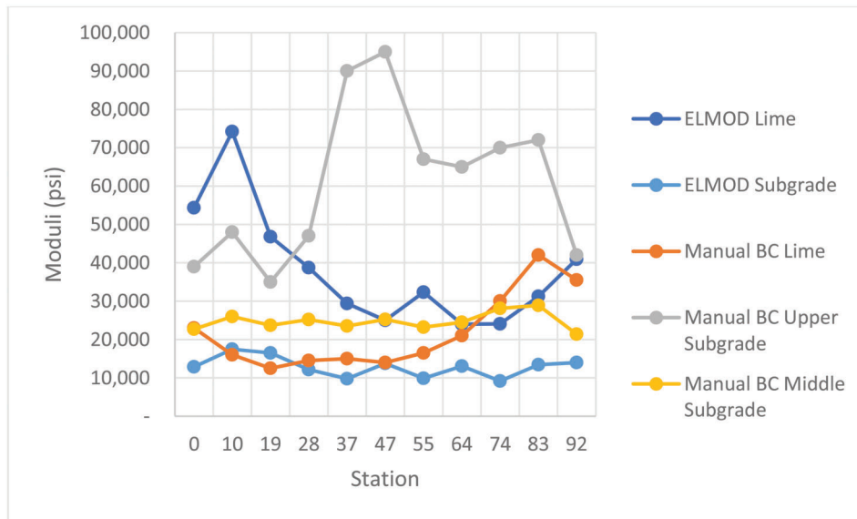
Figure A.8.6 Moduli of unbound layers, SR 37.
