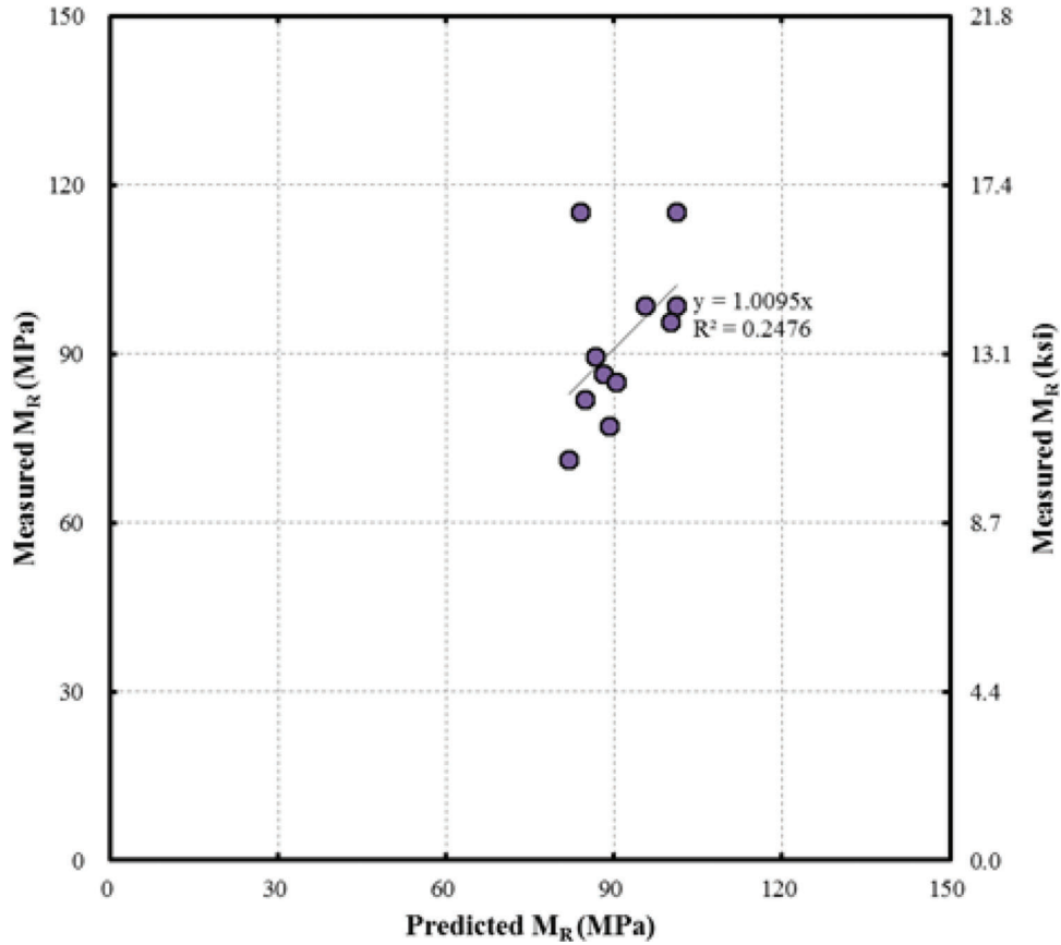
Figure A.5.3 Measured M_R vs Predicted M_R for A-7-6 soils (SR 37).
