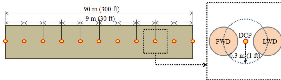
Figure 2.2 Schematic of selected section and test location.
