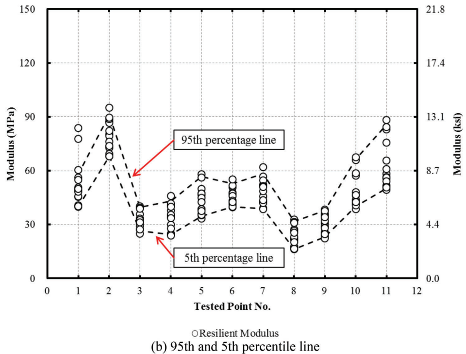
Figure 4.1 Range of resilient modulus values (US 31 site). (Figure continued next page.)
