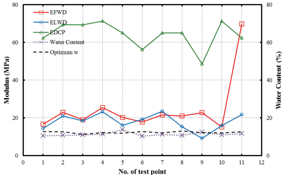
Figure A.3.12 E_{FWD} , E_{LWD} , E_{DCP} and water content of the subgrade at Ramp A.
