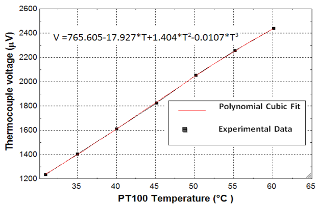
Fig.8: Variation of thermocouple voltage with reference PT100 sensor temperature
