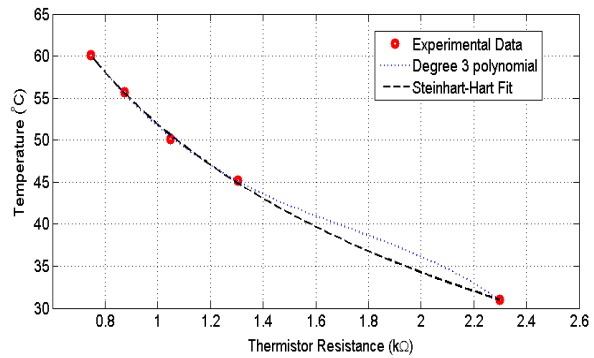
Fig.11: Cubic polynomial of Steinhart-Hart fit for the thermistor data.
