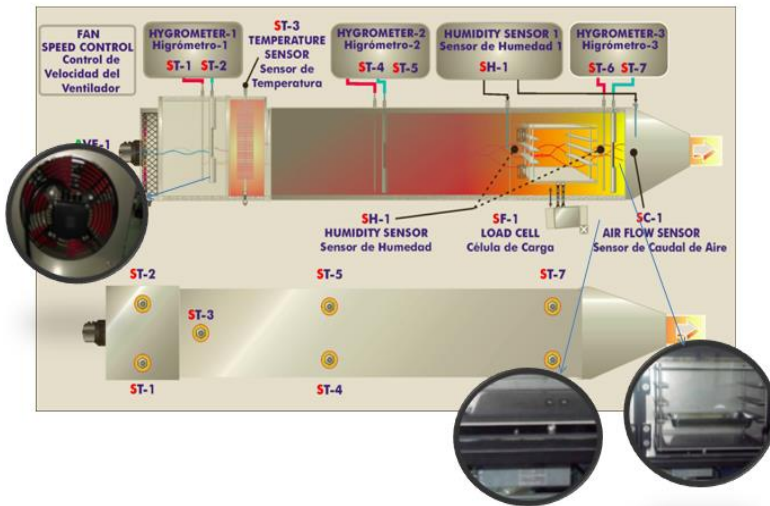
Fig.1a: Unit elements of computer controlled tray drier (Edibon) [16].
