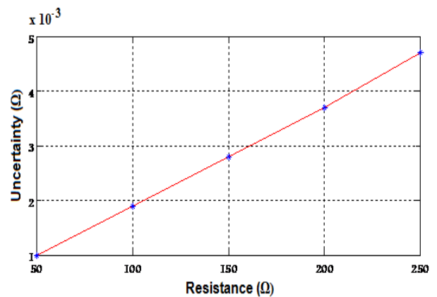
Fig.7: Variation of PT100IND resistance with uncertainty.
