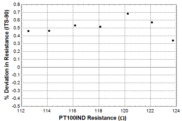
Fig.5: Variation of PT100IND resistance with percentage deviation in resistance (ITS-90).
