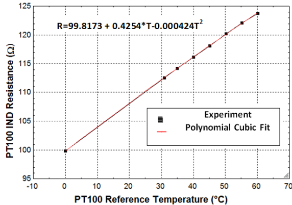
Fig.4: Variation of PT100 reference temperature with PT100IND resistance.
