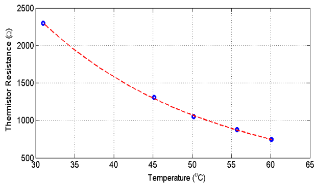
Fig.10: Variation of thermistor resistance with reference sensor temperature.
