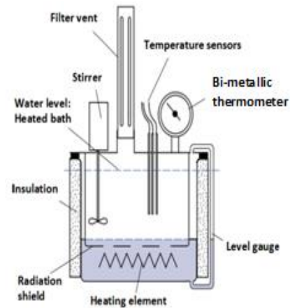
Fig.2: TH1 regulating bath [7,8].
