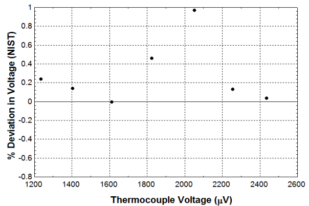
Fig.9: Variation of thermocouple voltage with percentage deviation in voltage (NIST).
