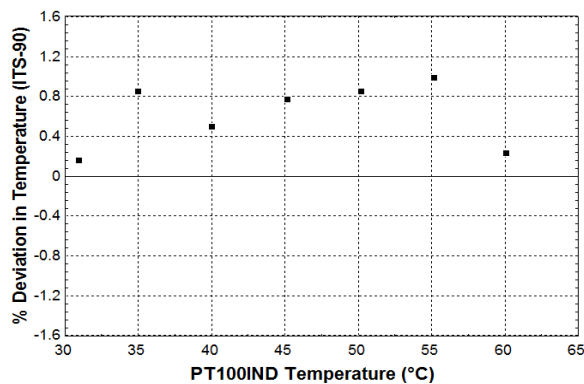
Fig.6: Variation of PT100IND temperature with percentage deviation in temperature (ITS-90).
