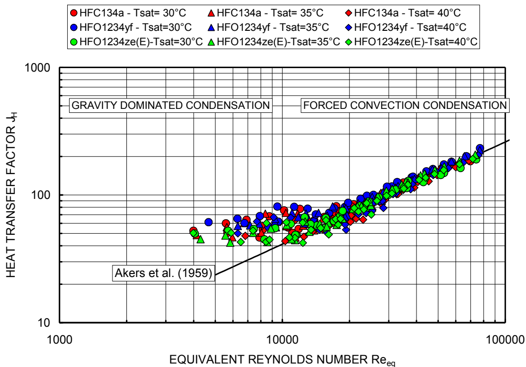
Figure 3: Experimental data plotted on the non-dimensional co-ordinates J_H vs. Re_{eq} .
