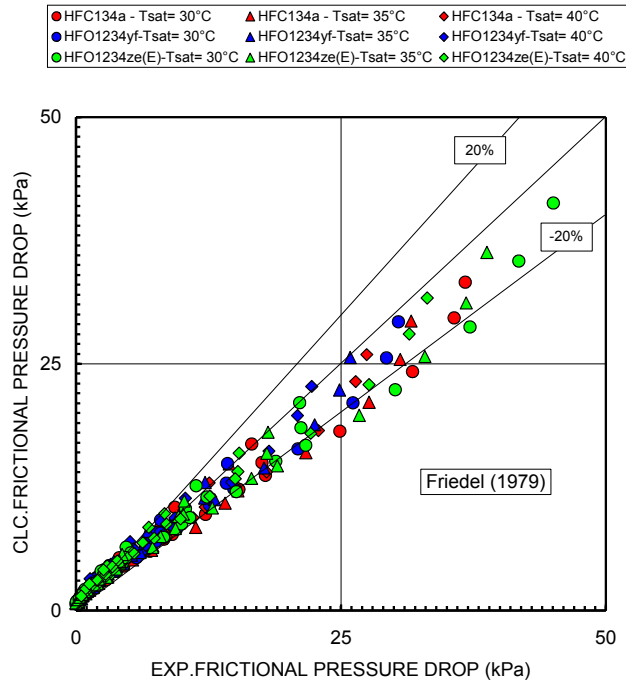
Figure 7: Comparison between experimental frictional pressure drop and calculated by Friedel (1979) equation.
