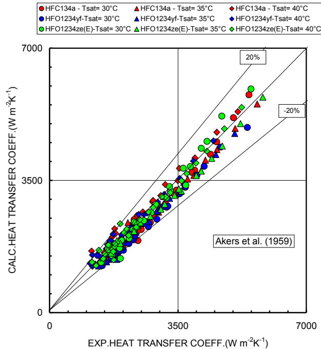
Figure 5: Comparison between experimental heat transfer coefficients and calculated by Akers et al. (1959) model.
