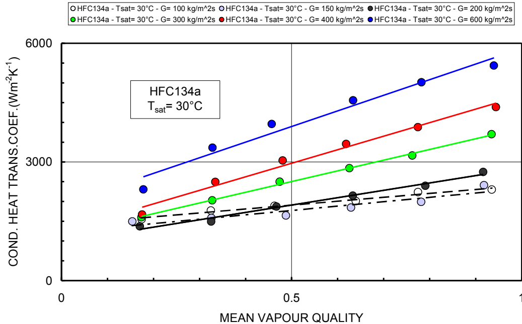
Figure 2a: Condensation heat transfer coefficient vs. mean vapour quality and mass flux at 30°C for HFC134a.
