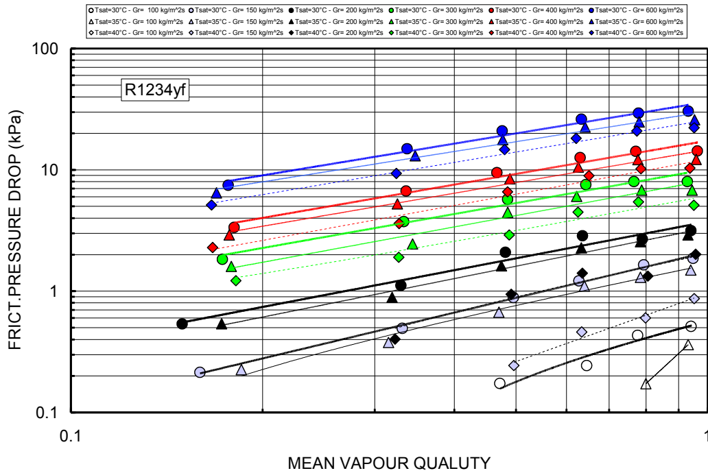
Figure 6b: Condensation frictional pressure drop vs. refrigerant mass flux for HFO1234yf.
