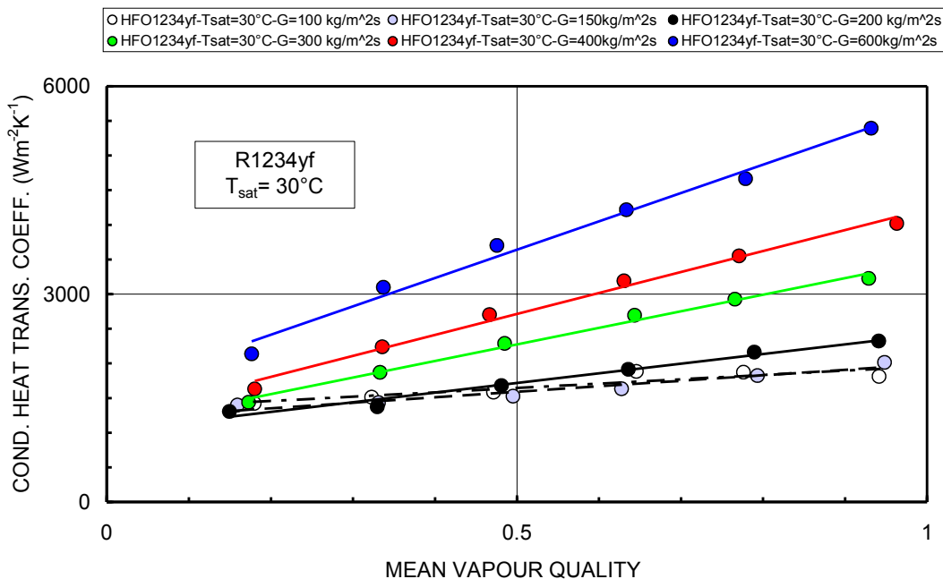
Figure 2b: Condensation heat transfer coefficient vs. mean vapour quality and mass flux at 30°C for HFO1234yf.
