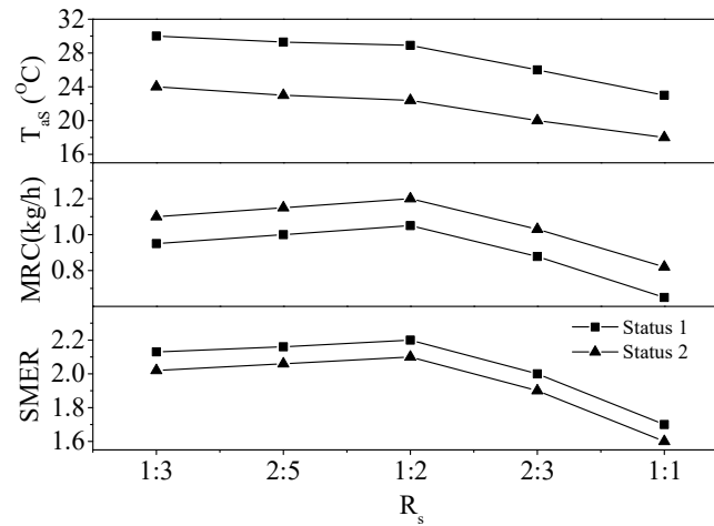
Figure 7: The operational characteristic of the EDAC system at ADO mode for the Case T-26 with different R_s values.
