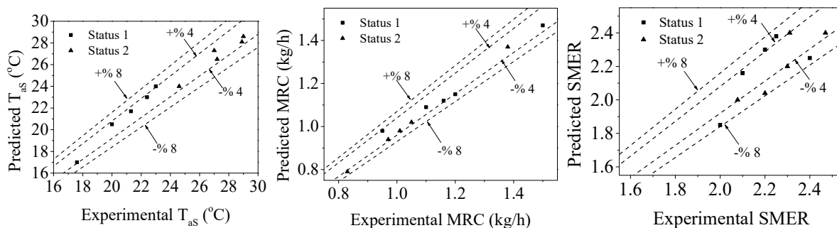
Figure 6: Modelled data versus experimental data
