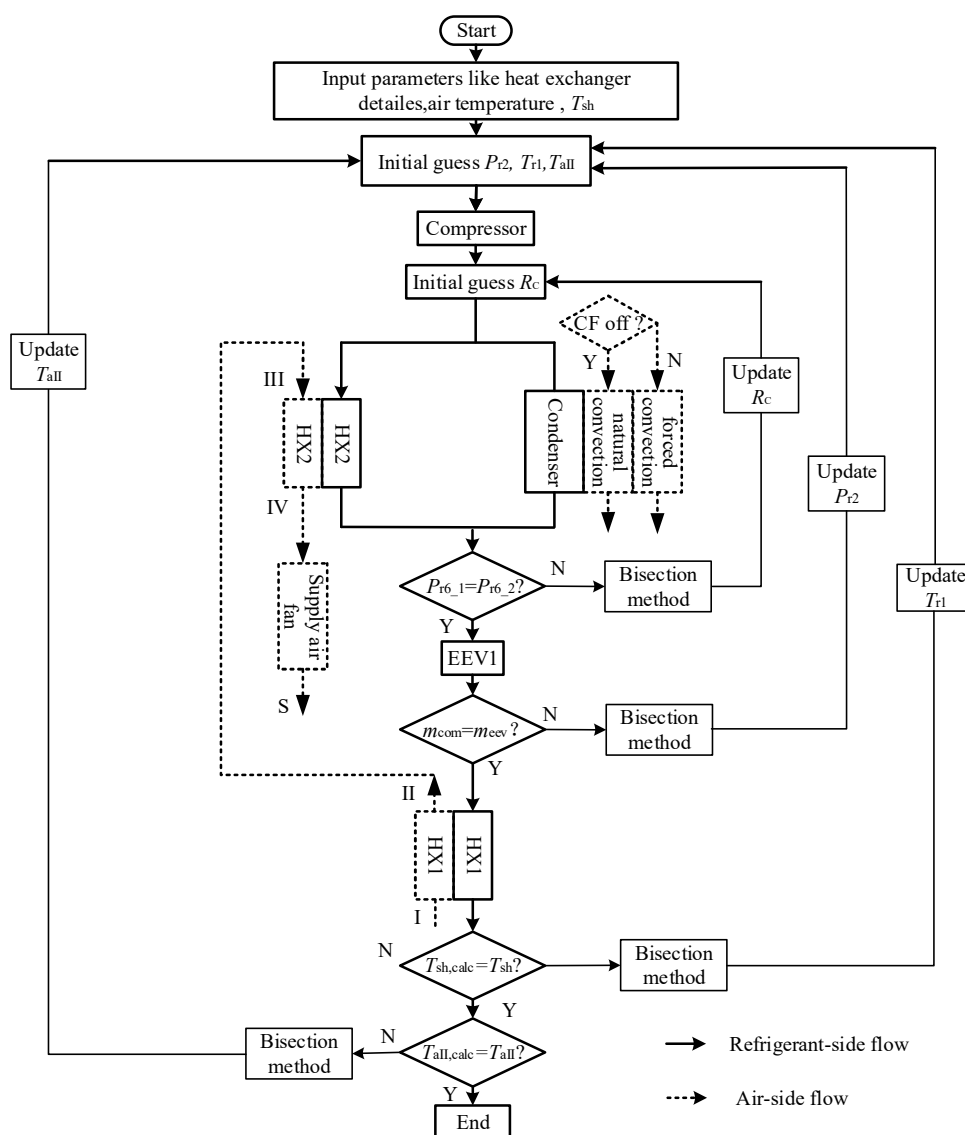
Figure 5: Flow chart of the calculation procedure of the complete EDAC system model for ADO mode
