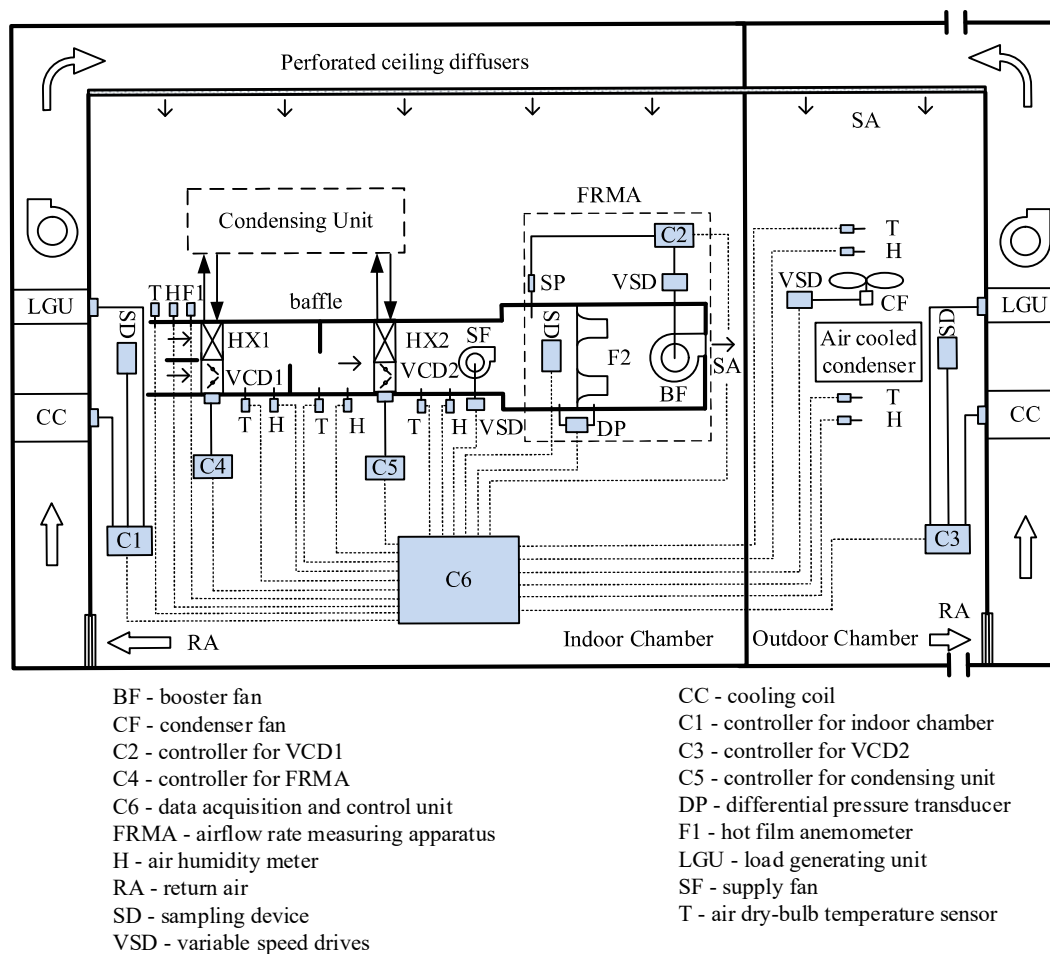
Figure 2: The schematic diagram of the prototype experimental EDAC system.
