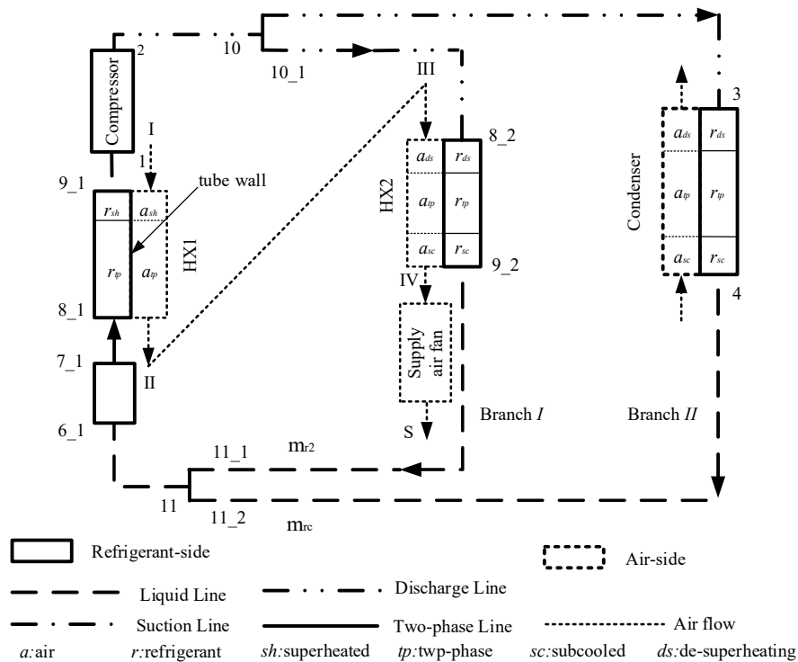
Figure 4: Conceptual model for EDAC system at ADO mode
