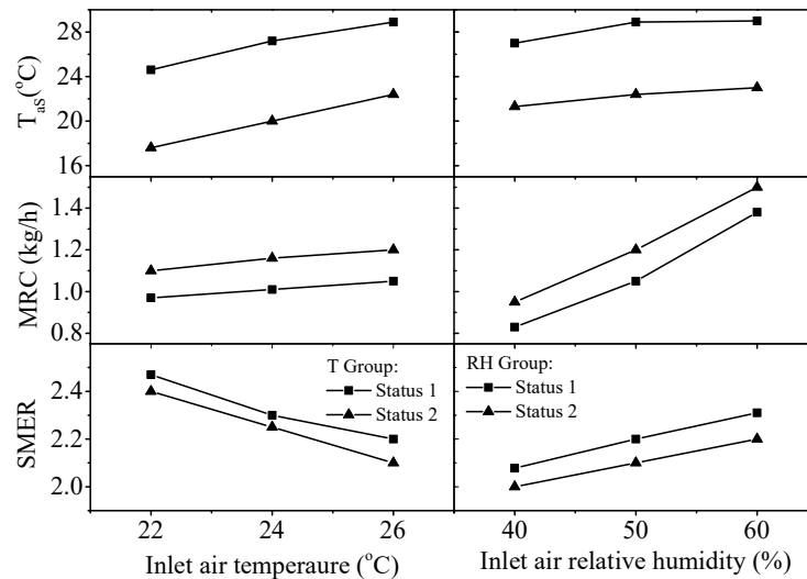
Figure 3: The influence of different indoor air states on the operational characteristics of the EDAC system at ADO mode
