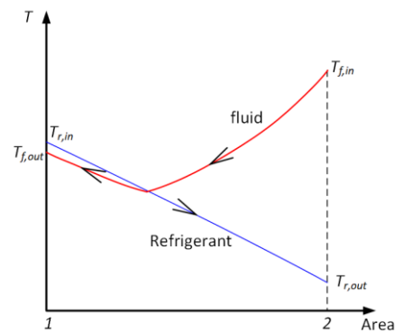
Fig. 14 Temp. crossing in a counter-flow evaporator
