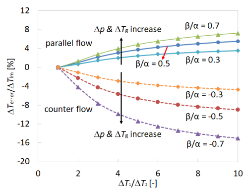
Fig. 6 Variations in LMTD error
