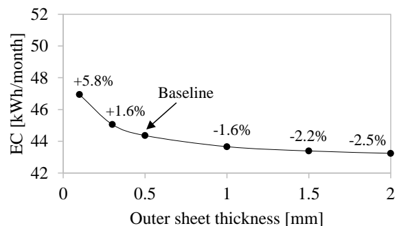
Figure 8: Energy consumption as a function of the outer sheet thickness
