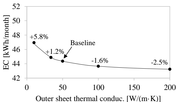
Figure 7: Energy consumption as a function of the outer sheet thermal conductivity
