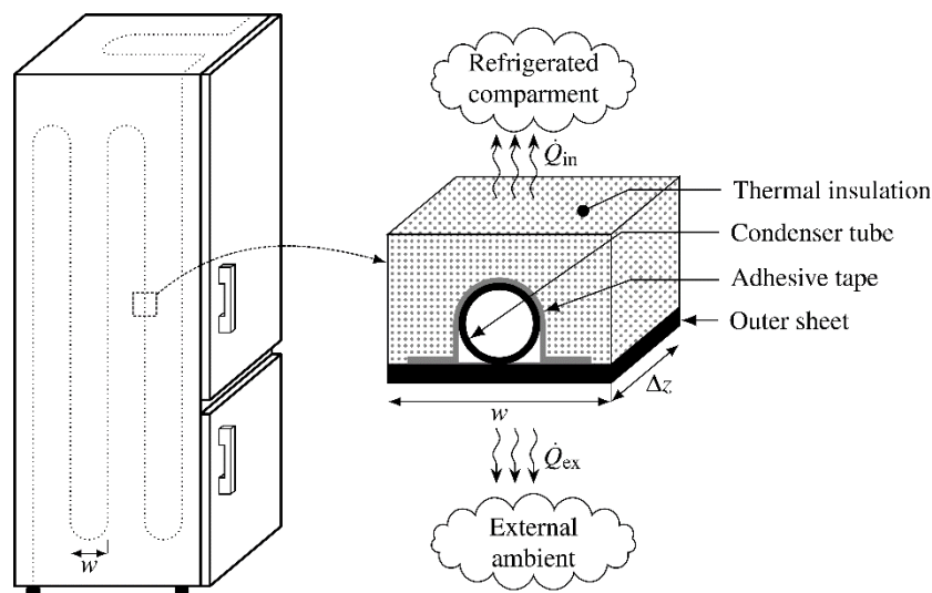
Figure 1: Condenser discretization
