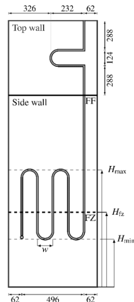
Figure 2: Sketch of the condensers circuitry
