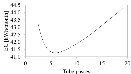
Figure 14: Energy consumption as a function of the number of tube passes
