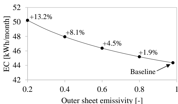
Figure 9: Energy consumption as a function of the outer sheet emissivity
