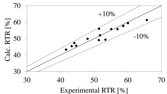
Figure 6: Validation of the run-time ratio
