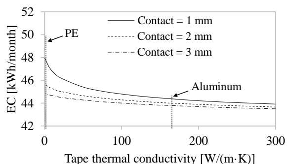
Figure 10: Energy consumption as a function of the tape thermal conductivity
