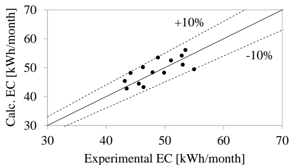
Figure 5: Validation of the energy consumption
