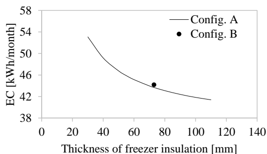
Figure 13: Energy consumption as a function of the thickness of the freezer insulation
